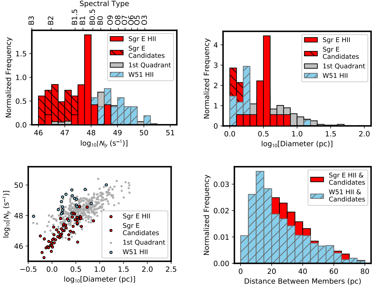
Figure 4. Comparison of the properties of the Sgr E and W51 HII regions, and the first quadrant HII region population from Makai et al. (2017) . The top left panel shows Lyman continuum photon rates derived from MeerKAT radio continuum data, the top right panel shows the HII region diameter distributions, the bottom left panel shows diameters versus Lyman continuum photon rates, and the bottom right panel shows the distances between members (known and candidate HII regions) of the complexes. In all panels, the distributions for the Sgr E sources are in red, the W51 sources are in blue, and the known HII region population is in grey. The Sgr E HII regions are less luminous on average compared to the W51 and first quadrant HII region populations, but have similar diameters, which implies that the age of the Sgr E HII regions is less than that of the first quadrant population, and much less than that of W51. The Sgr E HII regions and candidates are further apart from each other on average than those of W51.
