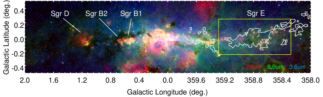
Figure 1. Spitzer three-color infrared view of the Galactic center region, with MIPS GAL 24 \mu\text{m} (red; Carey et al. 2009), GLIMPSE 8.0 \mu\text{m} (green; Benjamin et al. 2003; Churchwell et al. 2009), and GLIMPSE 3.6 \mu\text{m} (blue). Massive star formation regions have bright red 24 \mu\text{m} emission, and we identify some of these regions by name. White contours are of ^{13}\text{CO} 2 \rightarrow 1 emission (Schuller et al. 2017) integrated over velocity (Section 2.6) and the yellow box denotes the Sgr E complex.
