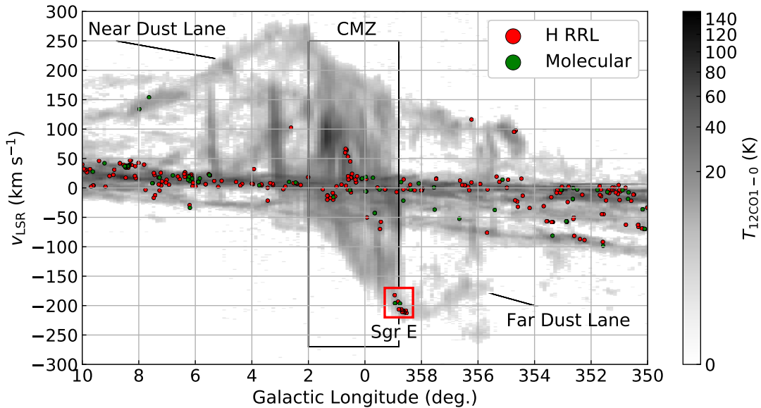
Figure 2. Longitude-velocity diagram of the inner Galaxy. The background is integrated ^{12}\text{CO} intensity (Dame et al. 2001), integrated over |b| < 1^\circ . WISE Catalog H II regions with measured hydrogen radio recombination line velocities are shown in red and those with only velocities of their associated molecular gas are shown in green. The black box highlights the nominal longitude zone of the CMZ: 2^\circ to -1.1^\circ . The red box highlights the zone used to define Sgr E in this work: 359.3^\circ > \ell > 358.3^\circ , -170 \text{ km s}^{-1} > v_{\text{LSR}} > -200 \text{ km s}^{-1} . The Sgr E H II regions are located at the intersection point of the far dust lane and the CMZ.
