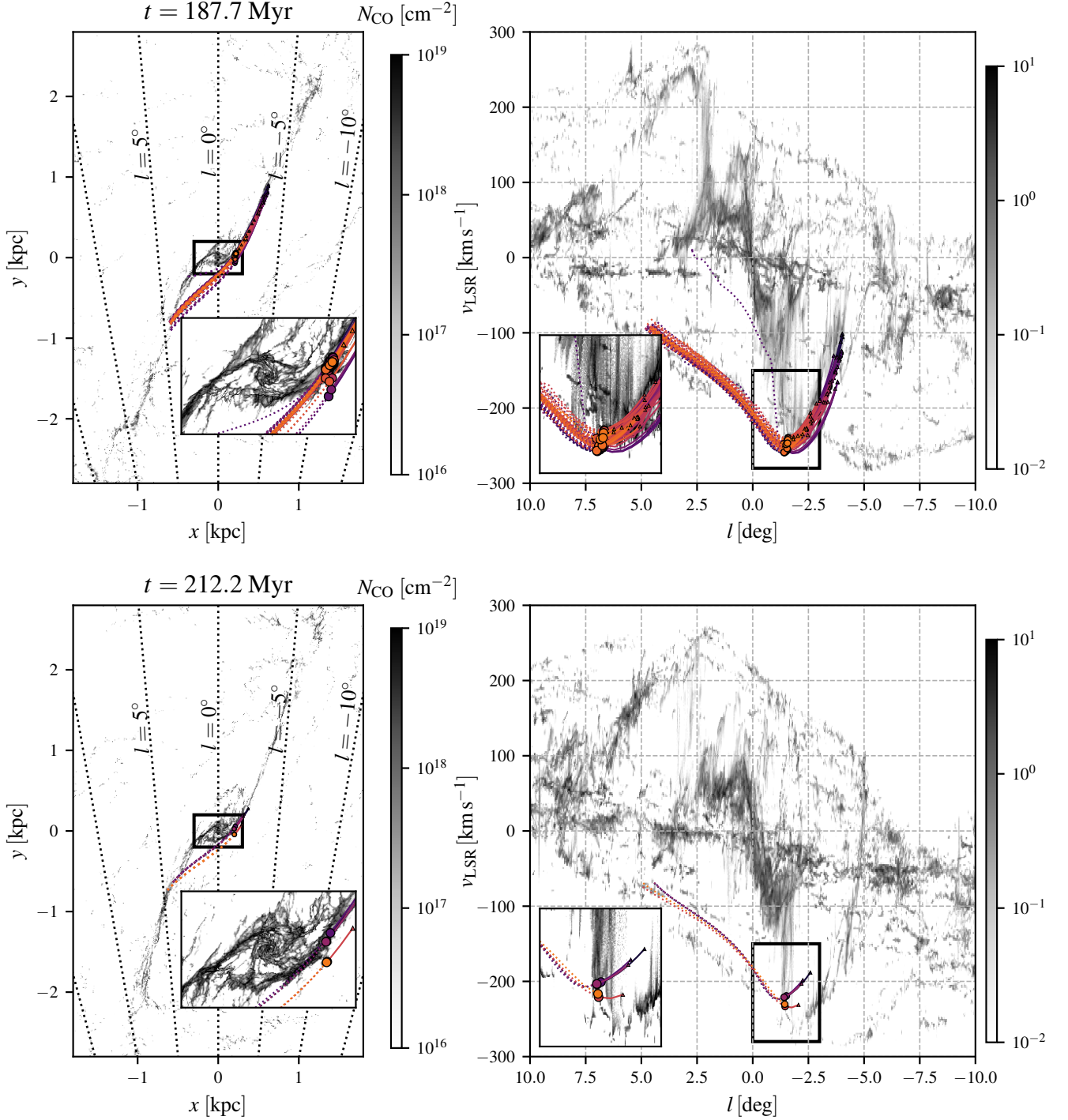
Figure 13. Newly born stars in two representative snapshots of the simulation presented in Tress et al. (2020) and Sormani et al. (2020) that lie in the zone 358.6^\circ > \ell > 358.4^\circ , have radial velocities v_{\text{LSR}} < -170 \text{ km s}^{-1} , and have distances from the Galactic center R \leq 300 \text{ pc} . Circles denote the positions of the stars in the snapshots and triangles indicate their birth sites. Solid lines show motion from the birth sites to their present locations and dotted lines show future motion for the next 5 Myr. The background grayscale image shows the distribution of molecular gas in the simulation, as traced by CO. The CO (\ell, v) projection is constructed using the simple method described in Section 3.6 of Sormani et al. (2018). The agreement between simulation and data is excellent (compare with Figures 2 and 12).
