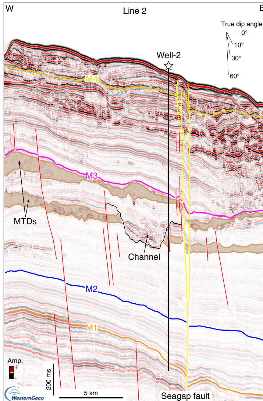
Fig. 4 Stratigraphy of the Tanzania margin imaged by a downslope-oriented seismic line crossing Well-2. Seismic Line 2, oriented W-E, crosses Well-2 offshore the northern Rovuma River delta. In this area, the oldest major mass-transport deposits (MTDs) accumulated during the Burdigalian (see Fig. 2 for the ages of the horizons). Noninterpreted version of Line 2 is available in the Supplementary Fig. 5.
