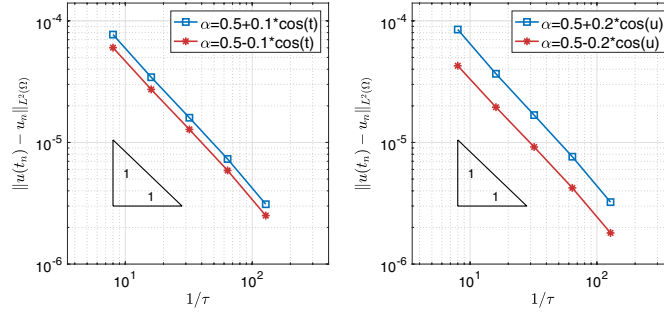
FIGURE 2. Errors of numerical solutions in Example 5.1.
