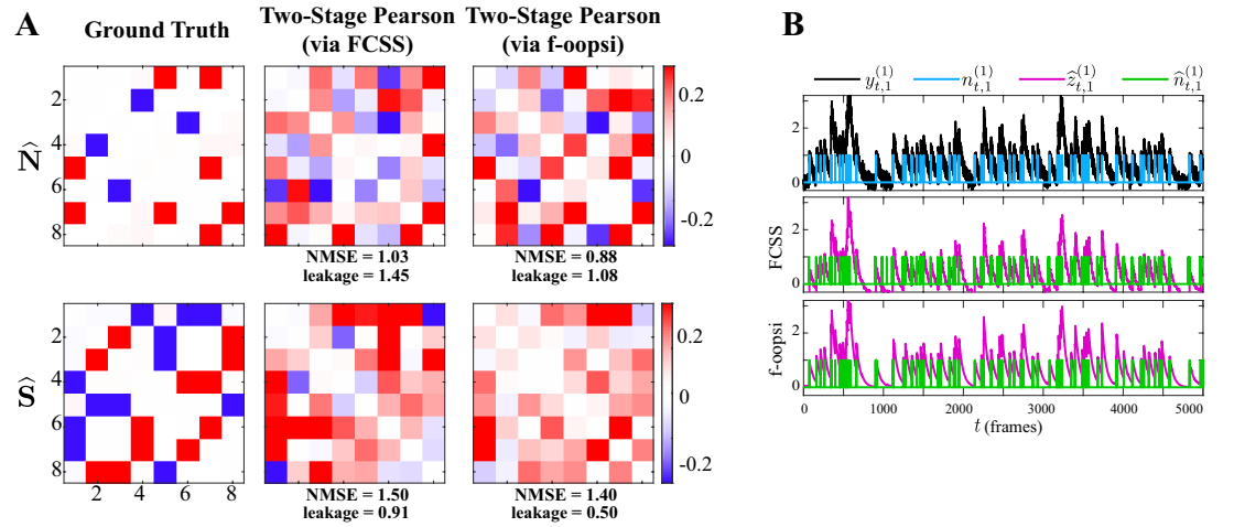
Figure 2-Figure supplement 1. A) Noise (first row) and signal (second row) correlations corresponding to the ground truth (first column), estimated by the two-stage Pearson method using the FCSS (Kazemipour et al., 2018) (second column) and constrained f-oopsi (Pnevmatikakis et al., 2016) (third column) spike deconvolution techniques, for the simulation study in Figure 2. The NMSE and leakage ratios of the estimates are indicated below each panel. While the correlation estimates based on these two methods are comparable, there exist notable differences between them, as a result of the slight discrepancies in the deconvolved spikes. This demonstrates that the two-stage estimates are sensitive to minor differences in the estimated spikes obtained by different deconvolution techniques. In addition, both two-stage Pearson estimates fail to capture the ground truth correlations (as is also evident from the high NMSE and leakage values). B) Simulated observations (black, re-scaled for ease of visual comparison) and ground truth spikes (blue), as well as the estimated calcium concentrations (purple) and putative spikes (green) for the 1 st trial of neuron 1 in the simulation study of Figure 2, using the FCSS (Kazemipour et al., 2018) (second row) and constrained f-oopsi (Pnevmatikakis et al., 2016) (third row) spike deconvolution methods.
