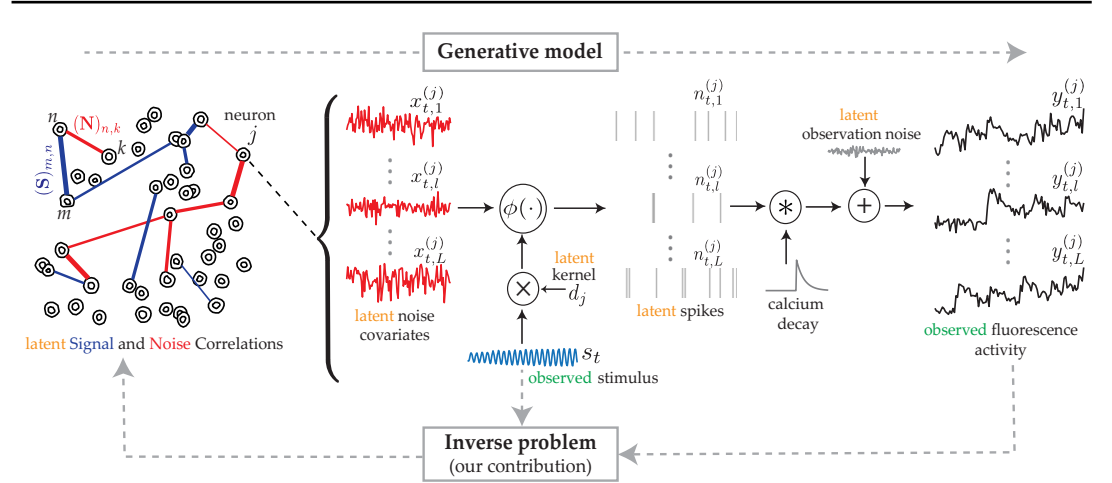
Figure 1. The proposed generative model and inverse problem. Observed (green) and latent (orange) variables pertinent to the j^{\text{th}} neuron are indicated, according to the proposed model for estimating the signal (blue) and noise (red) correlations from two-photon calcium fluorescence observations. Calcium fluorescence traces ( y_{t,l}^{(j)} ) of L trials are observed, in which the repeated external stimulus ( s_t ) is known. The underlying spiking activity ( n_{t,l}^{(j)} ), trial-to-trial variability and other intrinsic/extrinsic neural covariates that are not time-locked with the external stimulus ( x_{t,l}^{(j)} ), and the stimulus kernel ( d_j ) are latent. Our main contribution is to solve the inverse problem: recovering the underlying latent signal (S) and noise (N) correlations directly from the fluorescence observations, without requiring intermediate spike deconvolution.
