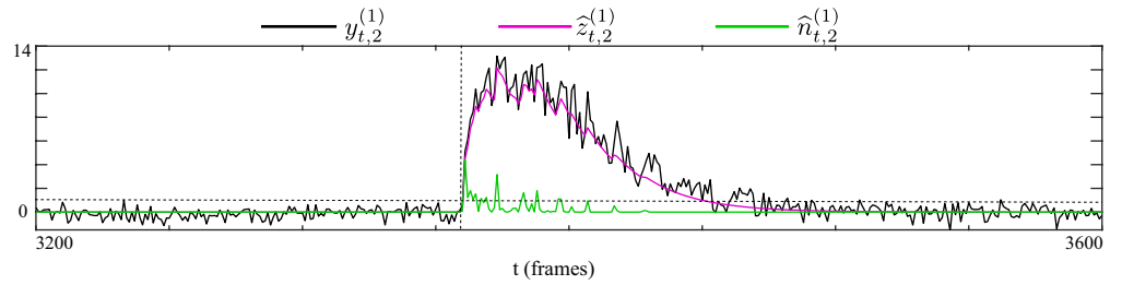
Figure 4-Figure supplement 2. The fluorescence observations (black), inferred calcium concentrations (purple) and putative spikes (green) by our proposed method, for a sample data segment with high fluorescence activity due to successive closely-spaced spikes. The rise onset of the fluorescence activity is marked by the vertical dashed line and spiking magnitude level of 1 is indicated by the horizontal dashed line. The proposed method favorably recovers the underlying calcium concentrations by predicting putative spikes in successive windows following the rapid rise of the fluorescence and with magnitudes possibly larger than 1.
