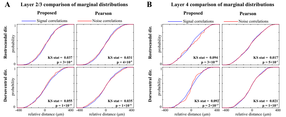
Figure 7-Figure supplement 1. Comparison of marginal distributions of signal and noise correlations. A) Cumulative marginal probability distributions of signal (blue) and noise (red) correlations along the rostrocaudal (top) and dorsoventral (bottom) directions, as estimated by the proposed method (left) and Pearson correlations from two-photon data (right), in layer 2/3 neurons. The Kolmogorov-Smirnov (KS) test statistic along with the corresponding p-values are indicated as insets in each panel. Panel B shows the results for layer 4 in the same organization as panel A. These results show that along both directions and in both layers, the signal correlation distributions are significantly different from the corresponding noise correlation distributions, consistently for both methods. However, the KS statistics (i.e., effect sizes) for the proposed estimate are remarkably larger than those obtained from the Pearson estimates.
