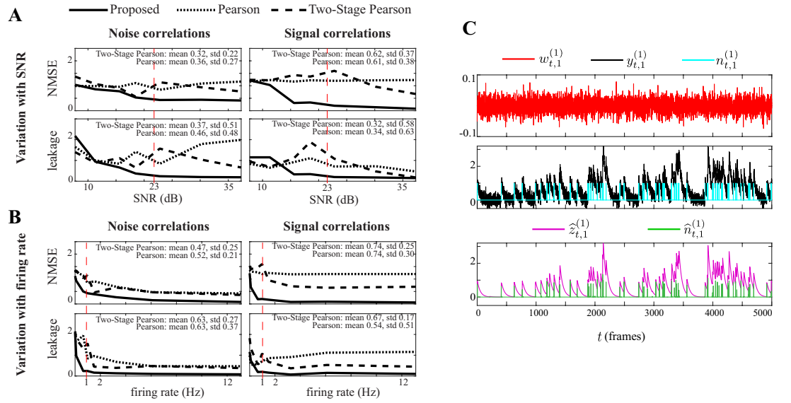
Figure 2-Figure supplement 5. Performance comparison with respect to varying SNR levels and average firing rates. A) NMSE (top) and leakage ratios (bottom) for the noise (left) and signal (right) correlation estimates vs. SNR (in dB), for the proposed method, Pearson correlations from two-photon data and Two-stage Pearson method. The SNR setting corresponding to Figure 2 is indicated by a dashed vertical line. The mean and standard deviation (std) of the normalized performance gain of the proposed method in comparison to the two existing methods are indicates as insets in each panel. B) Same organization as panel A, but with respect to varying firing rates (in Hz). C) Sample simulated white observation noise (red), two-photon observations (black, re-scaled for ease of visual comparison) and ground truth spikes (blue), as well as the estimated calcium concentrations (purple) and putative spikes (green) for the 1 st trial of neuron 1. While the performance of all methods degrade at low SNR levels or firing rates (SNR < 10 dB, firing rate < 0.5 Hz), our proposed method outperforms the existing methods for almost all SNR and firing rate settings considered.
