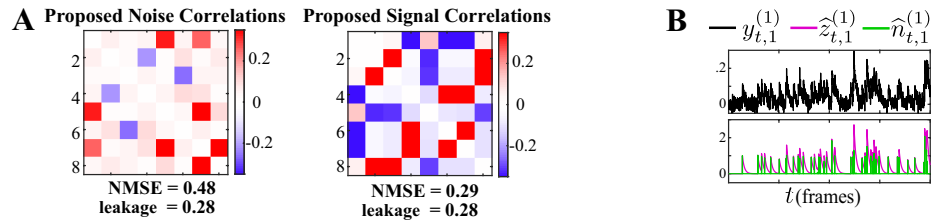
Figure 2-Figure supplement 4. A) Proposed noise and signal correlation estimates for data simulated at lower SNR than the setting of Figure 2 and model mismatch introduced by using a second-order autoregressive model for the calcium decay. The ground truth correlations are the same as those in Figure 2 . The NMSE and leakage ratio are given at the bottom. B) putative spikes (green) and estimated calcium concentrations (purple). The model mismatch and lower SNR result in slight performance degradation compared to Figure 2 (in terms of NMSE and leakage), and our method is capable of recovering the underlying correlations faithfully.
