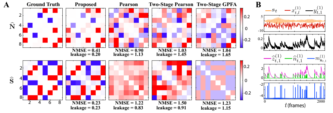
Figure 2. Results of simulation study 1. A) Estimated noise and signal correlation matrices from different methods. Rows from left to right: ground truth, proposed method, Pearson correlations from two-photon recordings, two-stage Pearson estimates and two-stage GPFA estimates. The normalized mean squared error (NMSE) of each estimate with respect to the ground truth and the leakage effect quantified by the ratio between out-of-network and in-network power (leakage) are indicated below each panel. B) Simulated external stimulus (orange), latent trial-dependent process (red), fluorescence observations (black), estimated calcium concentrations (purple), putative spikes (green) and estimated mean of the latent state (blue) by the proposed method, for the first trial of neuron 1.
