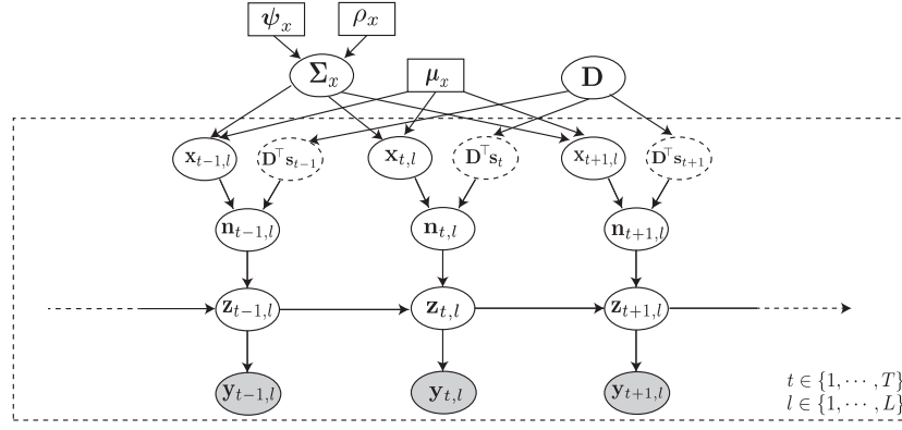
Figure 8. Probabilistic graphical model of the proposed forward model. The fluorescence observations at the t^{\text{th}} time frame and l^{\text{th}} trial: \mathbf{y}_{t,l} , are noisy surrogates of the intracellular calcium concentrations: \mathbf{z}_{t,l} . The calcium concentration at time t is a function of the spiking activity \mathbf{n}_{t,l} , and the calcium activity at the previous time point \mathbf{z}_{t-1,l} . The spiking activity is driven by two independent mechanisms: latent trial-dependent covariates \mathbf{x}_{t,l} , and contributions from the known external stimulus \mathbf{s}_t , which we model by \mathbf{D}^T \mathbf{s}_t (in which the receptive field \mathbf{D} is unknown). Then, we model \mathbf{x}_{t,l} as a Gaussian process with constant mean \mu_x , and unknown covariance \Sigma_x . Finally, we assume the covariance \Sigma_x to have an inverse Wishart prior distribution with hyper-parameters \psi_x and \rho_x . Based on this forward model, the inverse problem amounts to recovering the signal and noise correlations by directly estimating \Sigma_x and \mathbf{D} (top layer) from the fluorescence observations \{\mathbf{y}_{t,l}\}_{t=1,l=1}^{T,L} (bottom layer).
