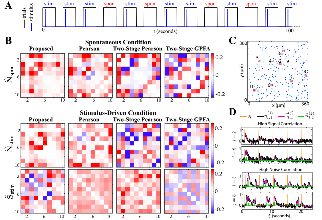
Figure 6. Comparison of spontaneous and stimulus-driven activity in the mouse A1. A) A sample trial sequence in the experiment. Stimulus-driven (stim) trials were recorded with randomly interleaved spontaneous (spon) trials of the same duration. B) Estimated noise and signal correlation matrices under spontaneous (top) and stimulus-driven (bottom) conditions. Rows from left to right: proposed method, Pearson correlations from two-photon data, two-stage Pearson and two-stage GPFA estimates. C) Location of the selected neurons with highest activity in the field of view. D) Stimulus onsets (orange), observations (black), estimated calcium concentrations (purple) and putative spikes (green) for the first trial from two pairs of neurons with high signal correlation (top) and high noise correlation (bottom), as identified by the proposed estimates.
