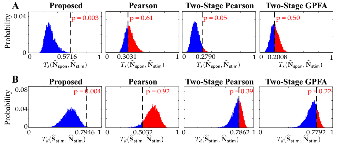
Figure 6-Figure supplement 1. Null distributions of A) the similarities between \hat{N}_{\text{spon}} and \hat{N}_{\text{stim}} (top: T_s(\hat{N}_{\text{spon}}, \hat{N}_{\text{stim}}) ) and B) the dissimilarities between \hat{S}_{\text{stim}} and \hat{N}_{\text{stim}} (bottom: T_d(\hat{S}_{\text{stim}}, \hat{N}_{\text{stim}}) ), obtained by the shuffling procedure applied to the results of real data study 2 in Figure 6 . The observed test statistic in each case is indicated by a dashed vertical line. Rows from left to right: proposed method, Pearson correlations from two-photon data, two-stage Pearson correlations and two-stage GPFA estimates. These results show that the only statistically significant outcomes (with p \leq 0.05 ) are the similarities and dissimilarities obtained by our proposed method.
