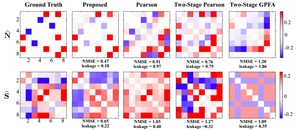
Figure 2-Figure supplement 3. Estimated noise and signal correlation matrices from different methods based on data generated with non-linear stimulus integration. Spikes were generated by replacing the linear receptive field model \mathbf{d}_j^T \mathbf{s}_t with a non-linear one given by \mathbf{d}_j^T \mathbf{s}_t + (\tilde{\mathbf{d}}_{j,1}^T \mathbf{s}_t)^2 + (\tilde{\mathbf{d}}_{j,2}^T \mathbf{s}_t)^2 , but a linear stimulus model was used for estimation (i.e., \tilde{\mathbf{d}}_{j,1} = \tilde{\mathbf{d}}_{j,2} = \mathbf{0} ). Rows from left to right: ground truth, proposed method, Pearson correlations from two-photon recordings, two-stage Pearson estimates and two-stage GPFA estimates. The normalized mean squared error (NMSE) of each estimate with respect to the ground truth and the leakage effect quantified by the ratio between out-of-network and in-network power (leakage) are indicated below each panel. While the NMSE in our proposed signal correlation estimates under this setting is greater than that in Figure 2 with no model mismatch, our proposed estimates still outperform existing methods. In addition, model mismatch in the stimulus integration component does not affect the accuracy of noise correlations estimated by our method.
