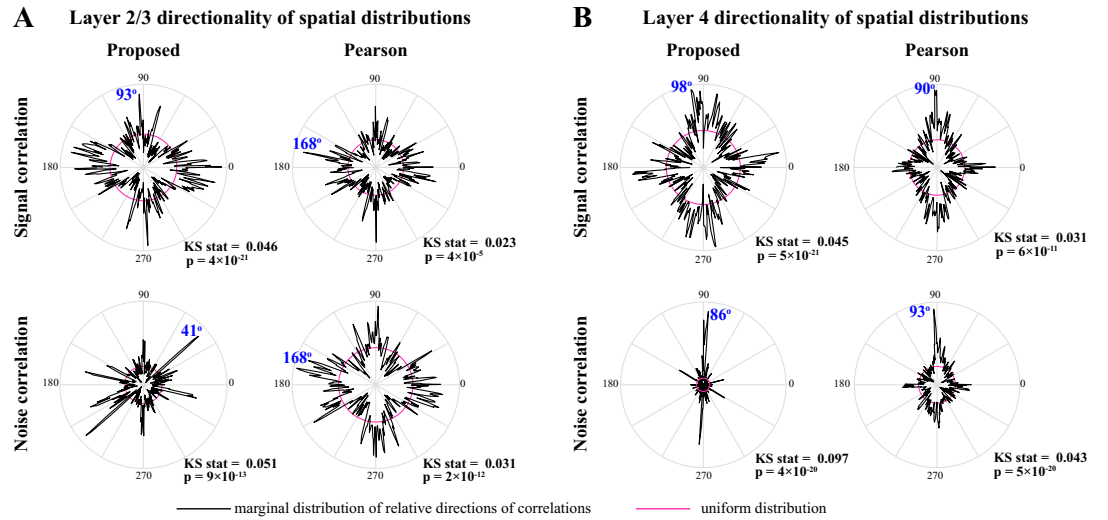
Figure 7—Figure supplement 2. Polar plots of the angular marginal distributions of correlations. A) Polar histograms indicating the distribution of signal (top) and noise (bottom) correlations as a function of relative angle (in the dorsoventral-rostrocaudal coordinate system) between pairs of neurons in layer 2/3, as estimated by the proposed method (left) and Pearson correlations from two-photon data (right). The KS test statistic comparing each polar distribution with a uniform distribution (shown in magenta), along with the corresponding p-values are indicated below each polar plot. The mode of each probability distribution is also indicated in blue fonts. Panel B shows the results for layer 4 in the same organization as panel A. All distributions are significantly non-uniform, and particularly indicate a rostrocaudal directionality in layer 4 (as indicated by the mode angles in panel B).
