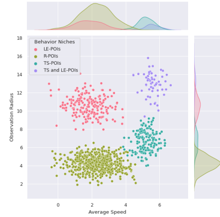
Figure 2: Discovered behavior niches in an environment with uniformly distributed R, TS and LE POIs. Niches with higher observation radii and lower speeds are optimal for LE POIs, whereas niches with higher average speeds are better suited for TS POIs.
