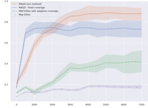
Figure 1: Fitness with uniformly distributed POIs. Our method promotes specialization of capabilities enabling agents to cooperate on diverse POIs. MAP-Elites struggles due to the need for learning the entire behavior repertoire.
