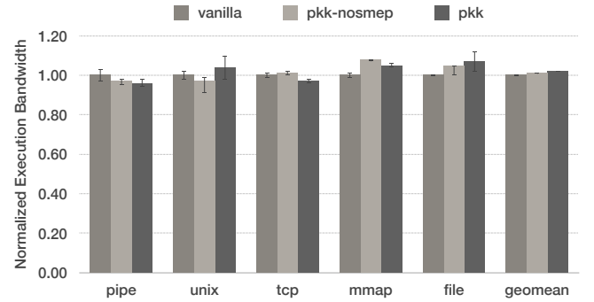
Figure 3: Breakdown of PKK overhead (over vanilla Linux) on LMBench bandwidth microbenchmarks. Columns labeled as pkk-nosmep represent IskiOS’s PKK implementation with the SMEP LLVM pass disabled.
