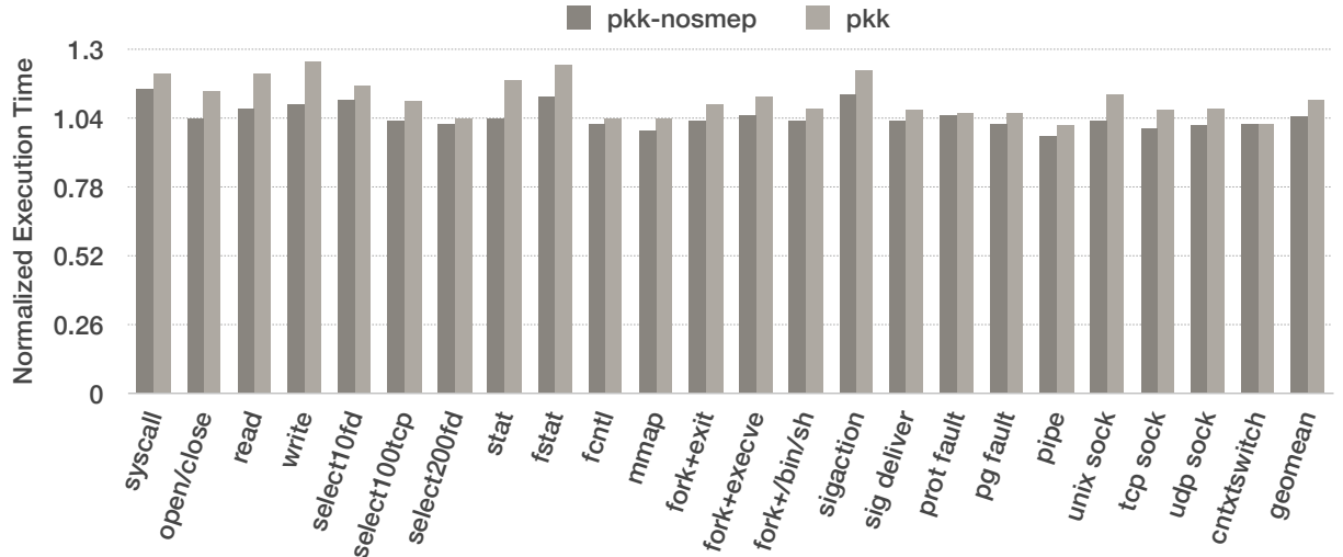
Figure 4: Breakdown of IskiOS’s PKK overhead (over vanilla Linux) on LMBench latency microbenchmarks. Columns labeled as pkk-nosmep represent IskiOS’s PKK implementation with the SMEP LLVM pass disabled.
