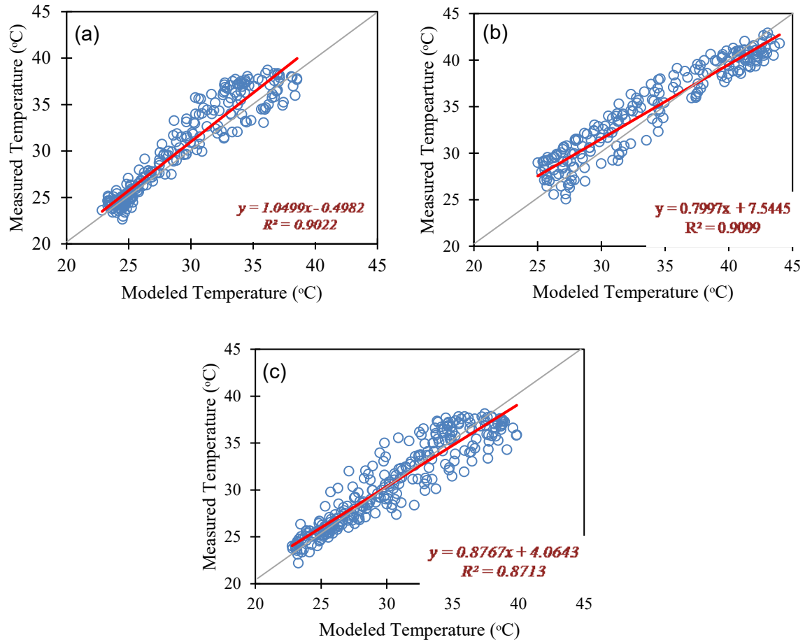
Figure 2. WRF/UCM hourly temperature results versus measured data during three heatwave events in Austin, TX, including (a) 8/8/2013, (b) 8/28/2011, and (c) 7/25/2017. (Note: grey line = 1:1; red line = bias correction linear regression line)
