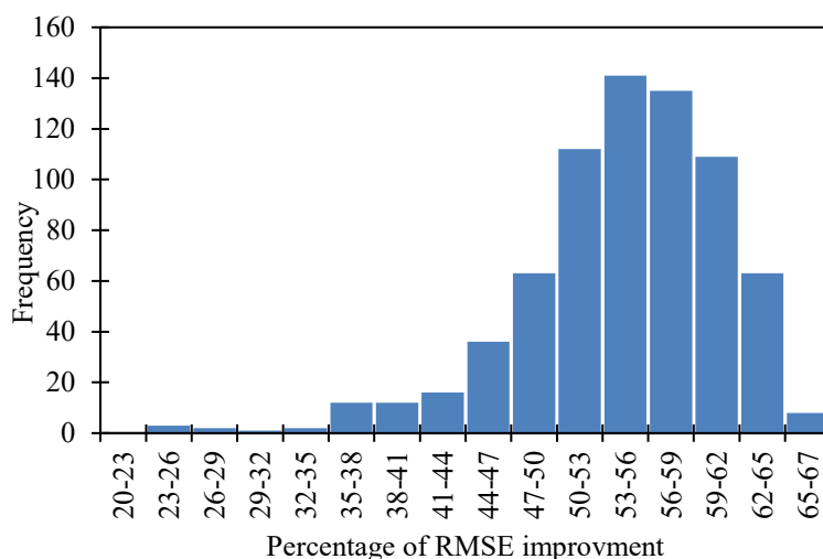
Figure 4. Percentage of RMSE improvement using the average delta correction method for 715 possible cases during the 8/28/2011 heatwave event
