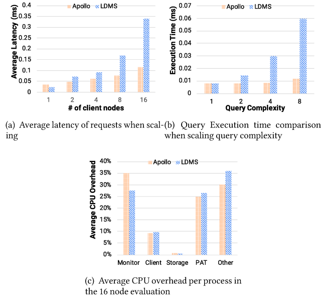
Figure 12: Comparison of Apollo and LDMS
