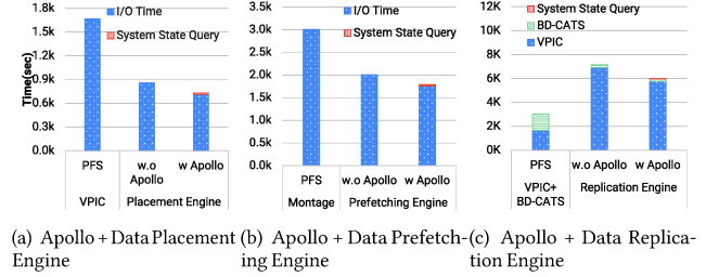
Figure 13: Apollo aiding middleware libraries
