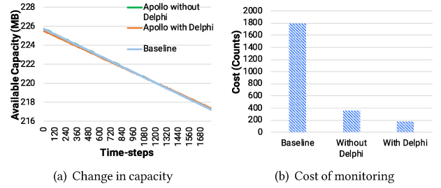
Figure 10: Apollo on regular HACC-IO workloads
