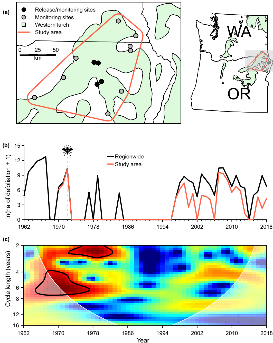
FIG. 1. (a) Map of 13 sites in Oregon (OR) and Washington (WA) where densities of larch casebearer and parasitism rates by Agathis pumila and Chrysocharis larinellae , two imported hymenopteran parasitoids, were tracked from 1972 to 1995. Sites are similarly mapped and described in Ryan (1990). (b) Time series of defoliation of western larch by larch casebearer in Oregon and Washington (1962–2018). Dashed vertical line indicates onset of biological control releases, and red line indicates defoliation within a convex hull polygon surrounding sites with a 10-km buffer (red polygon in maps of panel a). Data are from aerial detection surveys conducted by the U.S. Department of Agriculture Forest Service and state cooperators. Wasp graphic by Ben Davis from the Noun Project. (c) Wavelet analysis of defoliation data in (b) quantifying periodicity in population fluctuations. The colors of the contour indicate the power of the wavelet spectrum, with “red” indicating high power and increasingly “colder” colors indicating reduced power. The white shaded areas indicate the “cone of influence,” in which time-series edge effects become influential (Torrence and Compo 1998). The black lines in the graph enclose areas where the power of the spectrum was found to be significant.
