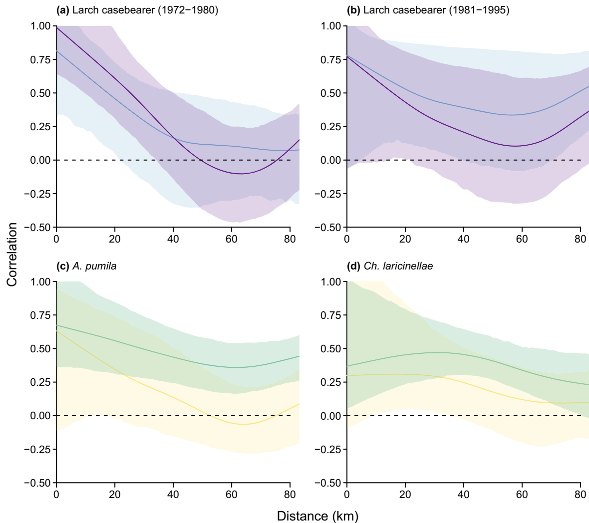
FIG. 3. Spatial synchrony quantified by spatial covariance functions of \ln(x + 0.001) -transformed densities (number per 100 buds) of larch casebearer larvae (blue) and adults (purple) from (a) 1972–1980 and (b) 1981–1995 and of A. pumila (c; yellow), and C. laricinellae (d; yellow) from 1981 to 1995 across 13 western larch sites in Oregon and Washington. Panels (c) and (d) also contain synchrony in parasitism rates pictured in green. Solid lines indicate mean synchrony in density or parasitism, and shaded areas are 95% confidence intervals. When confidence intervals include the dashed line, no statistically significant synchrony within insect densities was detected at the corresponding distance.
