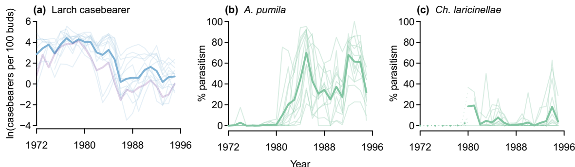
FIG. 2. Time series of (a) the number of larch casebearer larvae (blue line) and adults (purple line) per 100 buds and parasitism rates by (b) Agathis pumila and (c) Chrysocharis laricinellae across 13 western larch sites in Oregon and Washington (1972–1995). Dark lines are cubic smoothing splines fit to mean values for all sites, whereas lighter lines connect annual values at each site (site level lines not provided for casebearer adults). Corresponding dotted lines in panel (c) indicate spring parasitism rates prior to 1981, as winter parasitism rates, assumed to be approximately zero, were not available for several sites prior to 1981. A similar depiction of the data appear in Ryan (1997).
