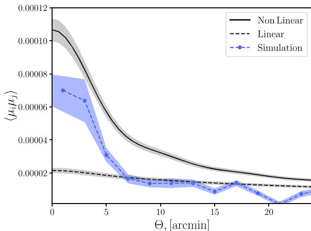
Figure 3. Measurements of the lensing correlation function measured from the MICE simulation to theoretical expectations from CAMB Sources. The solid black line is the expected correlation function assuming a non-linear power spectrum, and the black-dashed line assumes a linear power spectrum. The grey-shaded regions illustrate the one standard deviation regions of these functions, due to small differences in the redshift distributions of each realization. The blue hexagonal points illustrate the average measured lensing correlation function from the MICE simulation.
