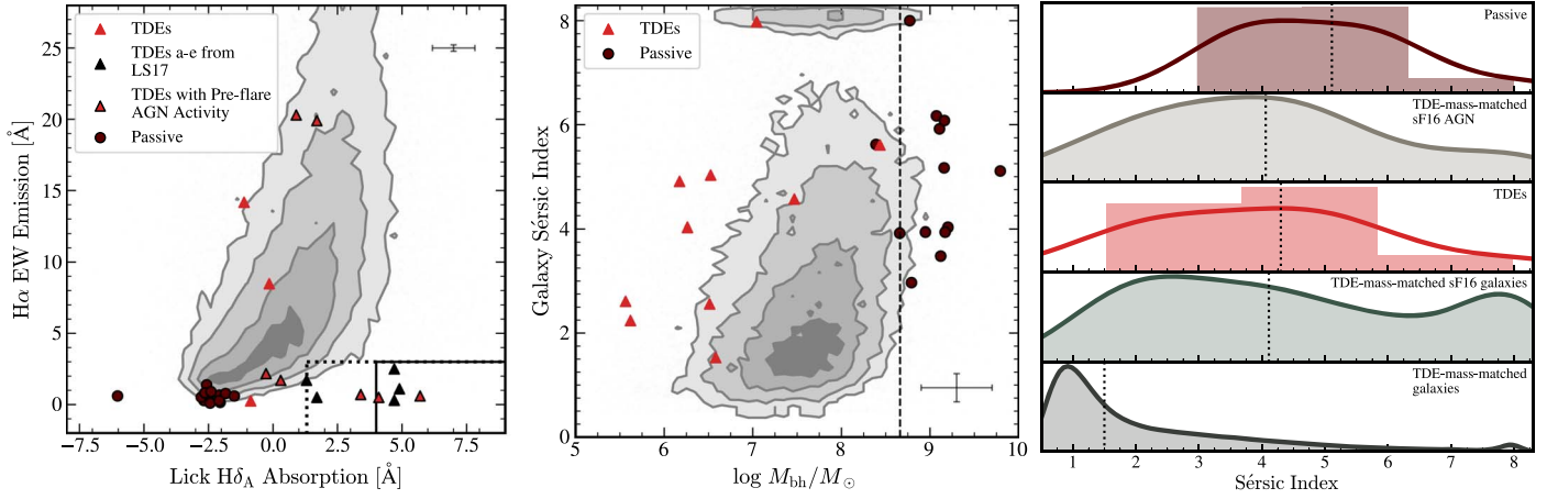
Figure 5. Left panel: H\alpha equivalent width vs. Lick H\delta absorption for Passive galaxies and TDEs, with AGNs as contours. TDEs with measured pre-flare AGN activity (French et al. 2020) are shown as red triangles outlined in black, and we additionally include TDEs a–e from LS17 as solid black triangles. As in Figure 1, solid black lines designate the E+A selection region, while the area between the dotted black lines shows the quiescent Balmer-strong region. Median error in measurements of Passive host galaxies is shown in the top right. Middle panel: Sérsic index vs. black hole mass for the same populations. The dashed line represents the upper limit on SMBH for a TDE to be visible for a Sun-like star and a maximally spinning SMBH ( a = 0.999 ), as calculated by Kesden (2012). At masses above this, tidal disruption would occur inside the event horizon. Median errors are shown in the bottom right. Right panel: smoothed and area-normalized histograms of Sérsic index. We compare the Passive galaxies and TDE hosts to a matched sample of galaxies and AGNs in the E+A box (sF16 selection) as well as all galaxies, with the added constraint that they have SMBH masses within the range of TDEs 1–5 (as defined in LS17). Median values are shown by dotted black lines.
