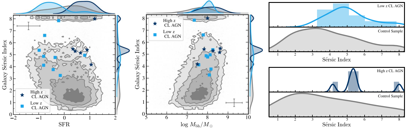
Figure 3. Left panel: Sérsic index vs. star formation rate for CL AGN hosts split by redshift, with low- z CL AGN hosts having 0.15 < z < 0.25 . Median errors for CL AGN hosts are displayed in the top left. 1D projections are smoothed and normalized to have areas of equal probability. Middle panel: Sérsic index vs. black hole mass for the same redshift groups of CL AGN hosts. Median errors are shown in the bottom right, and 1D projections are again smoothed and normalized. Right panel: histograms of Sérsic index for low- z CL AGNs (top) and high- z CL AGNs (bottom) with their respective control sample catalogs using the method developed by LS17, which are matched on SFR, total stellar mass, and redshift to a 7.5% tolerance. We note that this tolerance is larger than the one used by LS17 given the smaller number of AGNs as compared to regular galaxies.
