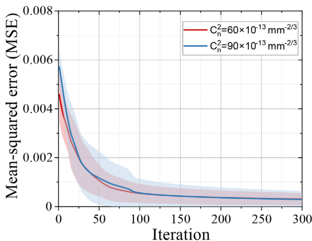
Figure 3. Mean-squared error (MSE) versus the iteration number in GDO. The red and blue lines indicate the MSE values for turbulence strengths C_n^2 = 60 \times 10^{-13} and 90 \times 10^{-13} \text{ mm}^{-2/3} , respectively. The number of iterations needed for the algorithm to achieve convergence depends on the strength of turbulence. In general, stronger turbulence requires longer times to converge.
