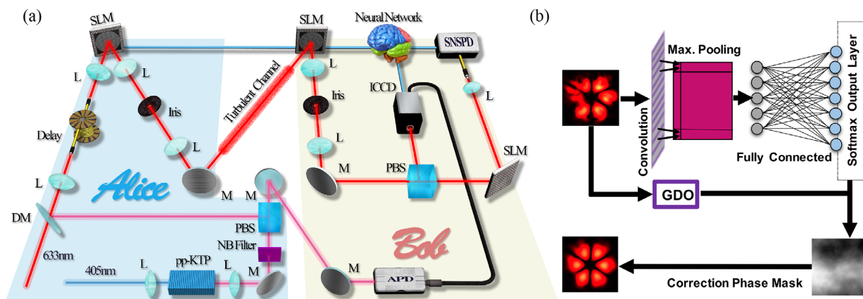
Figure 1. a) The schematic diagram of the setup used to demonstrate turbulence correction. The experiment is performed using a He-Ne laser and heralded single photons produced through a process of spontaneous parametric down-conversion (SPDC). The sources are switched using a dichroic mirror (DM). The spatial profile of photons is shaped by Alice using a spatial light modulator (SLM). The prepared photons are sent to Bob through a turbulent channel. Bob then performs correction and quantum state tomography on the structured photons. In order to do this, Bob collects multiple classical and single-photon images to train an artificial neural network. The high-light-level images are obtained with a CCD camera, whereas single-photon images are formed on a gated ICCD camera. b) The neural network for turbulence correction comprises a five-layer convolutional neural network (CNN), and a feedback loop with a gradient descent optimization (GDO) algorithm.
