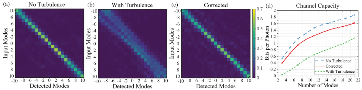
Figure 4. The cross-correlation matrices represent conditional probabilities between sent and detected modes in the OAM basis. a) The cross-correlation matrix obtained for our communication protocol in the absence of turbulence. b) Plot of the cross-correlation matrix in the presence of turbulence characterized by C_n^2 = 90 \times 10^{-13} \text{ mm}^{-2/3} . In this case, it is almost impossible to correctly identify the spatial modes. c) The cross-correlation matrix after applying our turbulence correction protocol. Our turbulence correction protocol significantly improves the performance of the communication system. d) Channel capacity in terms of bits per photon.
