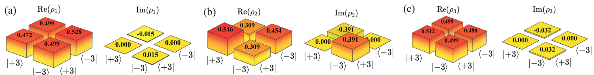
Figure 5. Real and imaginary parts of the density matrices for the qubits encoded in the OAM basis. In this case, we prepared |\psi_3\rangle = \frac{1}{\sqrt{2}}(|\text{LG}_{+3,0}\rangle + |\text{LG}_{-3,0}\rangle) . a) The real and imaginary parts of the density matrix for the undistorted state. b) The density matrix for the aberrated qubit. In this case, the strength of the simulated turbulence is characterized by C_n^2 = 80 \times 10^{-13} \text{ mm}^{-2/3} . c) The density matrix for the corrected qubit after applying our turbulence correction protocol. We measured a fidelity of 99.9% for the prepared state, 81.7% for the distorted state, and 99.8% for the state corrected through our machine learning protocol.
