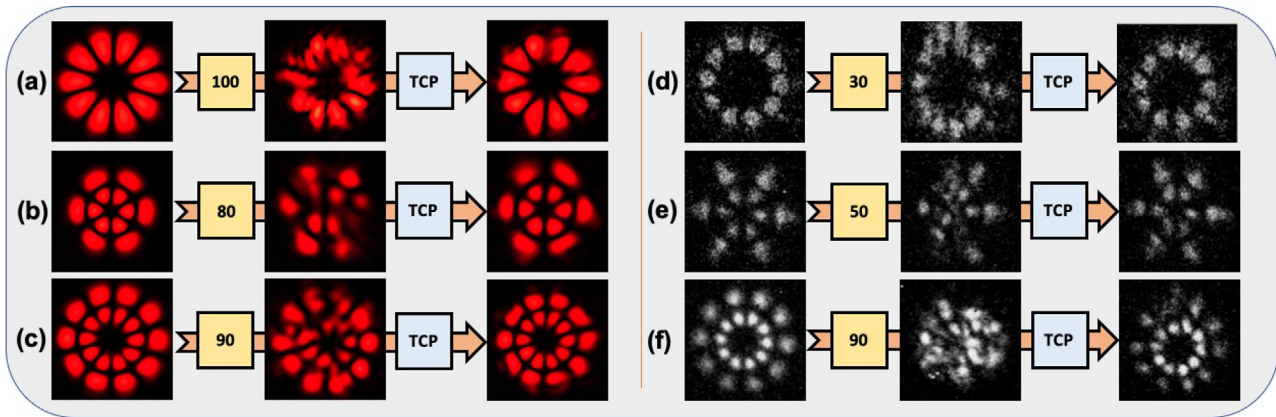
Figure 2. Spatial profiles of LG modes at high- and single-photon levels for different turbulence conditions. The first column in each of the panels shows the states prepared by Alice without distortions. The second columns display the distorted beams measured by Bob. The strength of turbulence is characterized by C_n^2 ( \times 10^{-13} \text{ mm}^{-2/3} ), these numbers are reported in the yellow rectangle. The spatial profiles after our turbulence correction protocol (TCP) are shown in the third column. a–c) High-light-level demonstrations of our protocol for multiple LG superpositions, |\psi\rangle = \frac{1}{\sqrt{2}}(|\text{LG}_{+5,0}\rangle + |\text{LG}_{-5,0}\rangle) , |\psi\rangle = \frac{1}{\sqrt{2}}(|\text{LG}_{+3,1}\rangle + |\text{LG}_{-3,1}\rangle) , and |\psi\rangle = \frac{1}{\sqrt{2}}(|\text{LG}_{+5,1}\rangle + |\text{LG}_{-5,1}\rangle) , respectively. d–f) The corresponding single-photon demonstrations of (a), (b), and (c), respectively.
