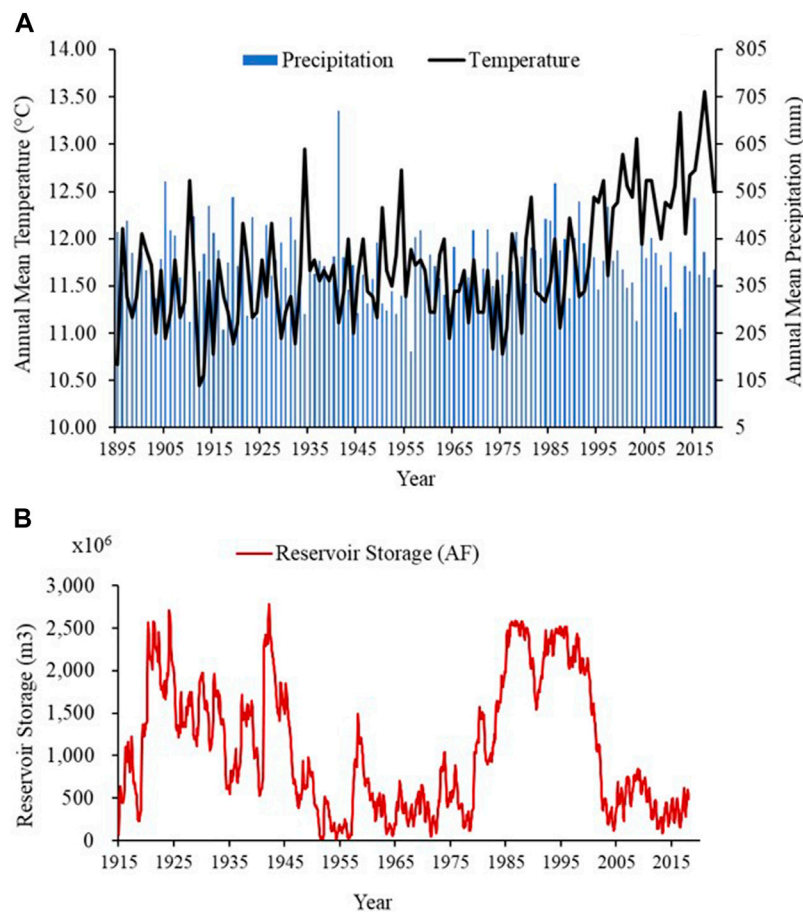
FIGURE 7 | (A) Annual mean precipitation and temperature of the United States and New Mexico from 1895 to 2019 (Source: www.ncdc.noaa.gov/temp-and-precip/ ) and (B) Elephant Butte Reservoir storage levels ( \text{m}^3 ) in New Mexico from 1915 to 2020 (Source: USBR, 2021).
