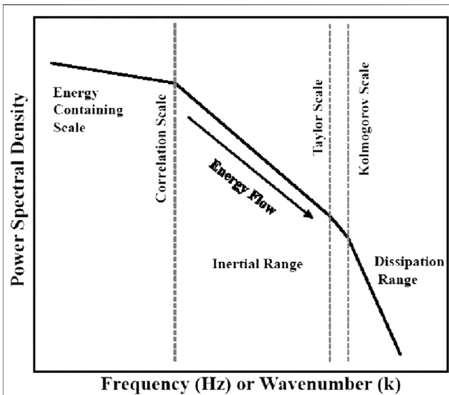
FIGURE 1 | Schematic of a typical power spectral density plot for turbulent solar wind. The lowest frequencies are at the energy containing scales and the dissipation range is at the highest frequencies. The correlation scale (left most dashed gray line) separates energy containing scales and the inertial range while the Kolmogorov scale (right most dashed gray line) is between the inertial range and the dissipation range. The third scale on the schematic is the Taylor scale (middle dashed gray line), the scale at which eddies start to damp out, (Adapted from Goldstein et al. (1995)).
