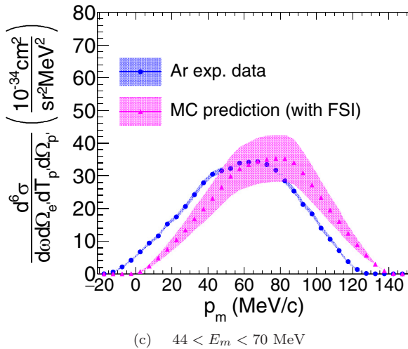
FIG. 7. Sixfold differential cross section for argon as a function of missing momentum integrated over different ranges of missing energy. The background estimate is multiplied by 10 for presentation. The MC predictions, based on the mean-field SF, include the full FSI corrections.
