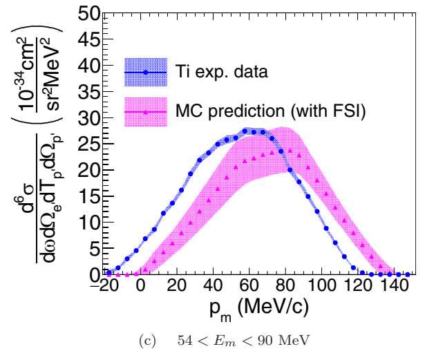
FIG. 8. Same as Fig. 7 but for titanium.
