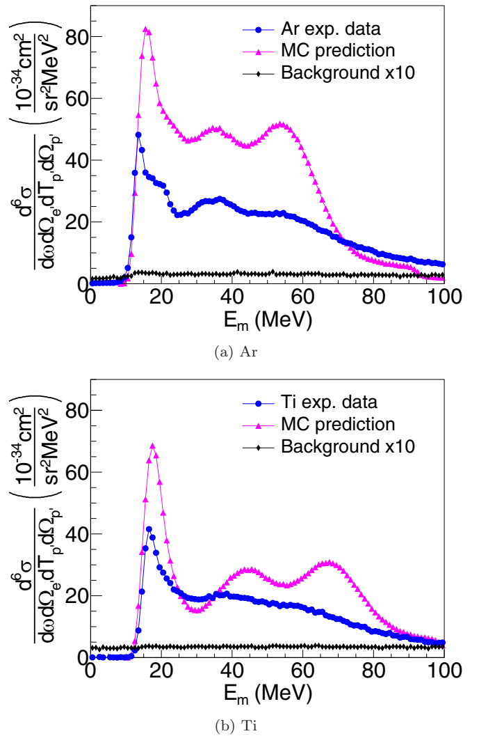
FIG. 3. Sixfold differential cross section as a function of missing energy for argon (a) and titanium (b). The background estimate (line connecting the experimental data points) is multiplied by 10 for purpose of presentation. The MC predictions, based on the mean-field SF, include a correction for the nuclear transparency, while other FSI effects are not accounted for.
