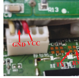
Fig. 8. UART of WeMo plug
