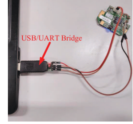
Fig. 9. Open a console of WeMo plug system by UART
