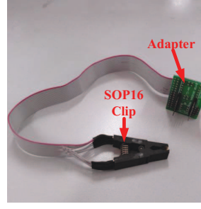
Fig. 5. Adapter and SOP16 Clip
