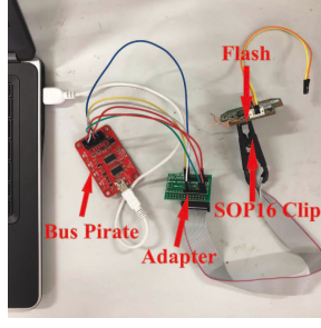
Fig. 4. Reading Flash by Bus Pirate
