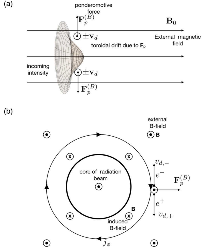
FIG. 1. (a) View from the side. An intense radiation beam is propagating along the magnetic field. The gradients of the field intensity induce the ponderomotive force \mathbf{F}_p^{(B)} . In the high external magnetic field B_0 the ponderomotive force leads to azimuthal drift of charged particles \pm \mathbf{v}_d that creates toroidal current and decreases the background magnetic field. (b) View along the direction of the beam. In the core the radiation energy density is high and it induces a ponderomotive force directed away from the center. In the external magnetic field (chosen to be out of the plane) the ponderomotive force leads to charge-dependent drift of particles and generation of the toroidal current (in the clockwise direction). The induced current produces a field counteraligned with the external field.
