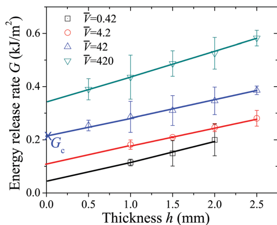
Fig. 4 Energy release rate as a function of thickness of the films with different normalized crack velocities \bar{V} .
