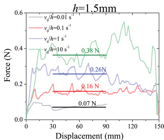
Fig. 3 Force vs. displacement of tear experiments with the film thickness of 1.5 mm.
