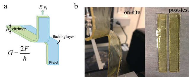
Fig. 2 (a) A schematic of tear test: one arm is fixed, and the other arm is stretched at a speed of v_0 . (b) Tearing the vitrimer and the torn vitrimer with a smooth crack surface.
