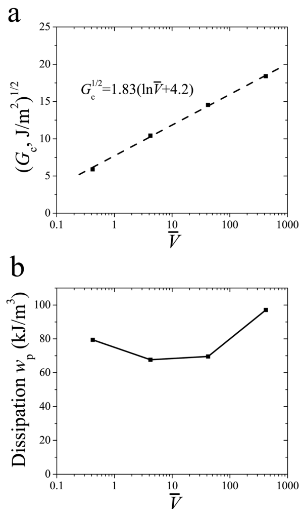
Fig. 5 (a) The intrinsic fracture energy as a function of the normalized crack velocity, where the intrinsic fracture energies are the intercepts of the lines with vertical axis in Fig. 4; (b) bulk dissipation of vitrimer with different normalized crack velocities, where bulk dissipation is the slopes of the lines in Fig. 4.
