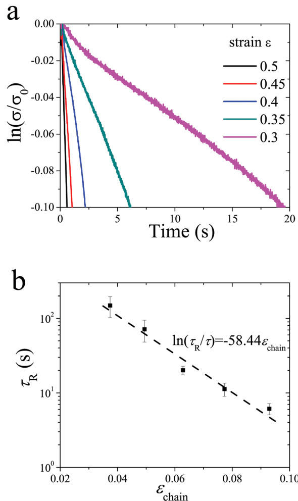
Fig. 6 (a) Stress relaxation of a vitrimer with different applied strains \varepsilon . (b) Relaxation time as a function of the chain strain \varepsilon_{\text{chain}} .
