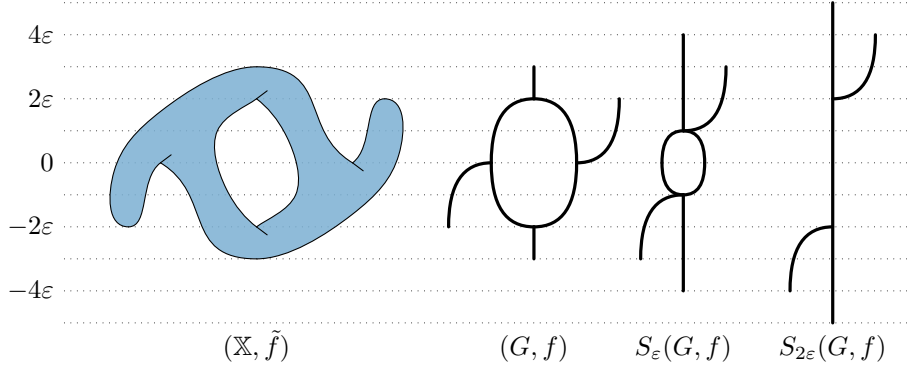
■ Figure 1 From left to right: an \mathbb{R} -space (\mathbb{X}, \tilde{f}) , its Reeb graph (G, f) , smoothings are shown for two parameters, \varepsilon and 2\varepsilon . Function values are shown by height.
