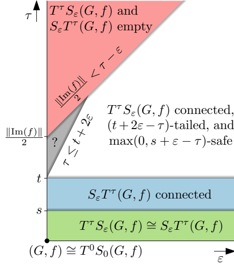
■ Figure 7 For connected, t -tailed, and s -safe (G, f) , properties of S_\epsilon^\tau(G, f) = T^\tau S_\epsilon(G, f) and S_\epsilon T^\tau(G, f) , parameterized by \tau and \epsilon .
