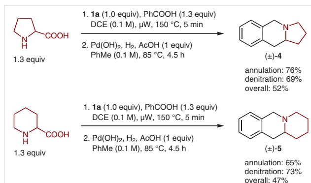
Scheme 6 Decarboxylative annulation/denitration
