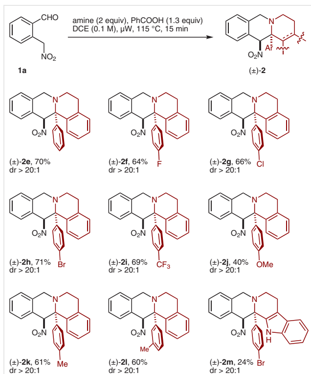
Scheme 4 Formation of sterically congested tetrahydroprotoberberine analogues
