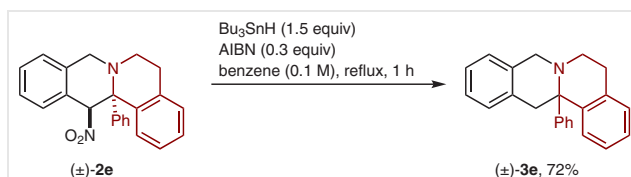
Scheme 5 Denitration of a sterically congested annulation product
