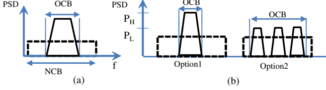
Fig. 5. (a) Relation between OCB and NCB, (b) examples of NR-U interlace waveform designs (option 1 does not meet the FCC OCB/NCB requirement, but option 2 does).
