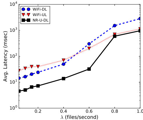
Fig. 23. Average latency vs. \lambda (indoor at 6.18 GHz; transmit power: 18 dBm; channel bandwidth: 20 MHz; 3GPP InH path loss model).
