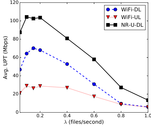
Fig. 21. Average UPT vs. \lambda (indoor at 6.18 GHz; transmit power: 18 dBm; channel bandwidth: 20 MHz; 3GPP InH path loss model).
