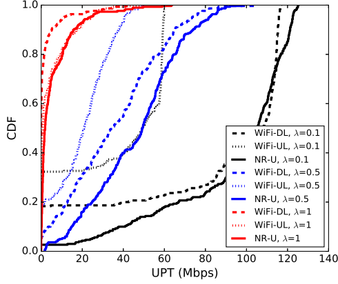
Fig. 12. CDF of UPT (indoor at 5.18 GHz; transmit power: 23 dBm; channel bandwidth: 20 MHz; 3GPP InH path loss model).
