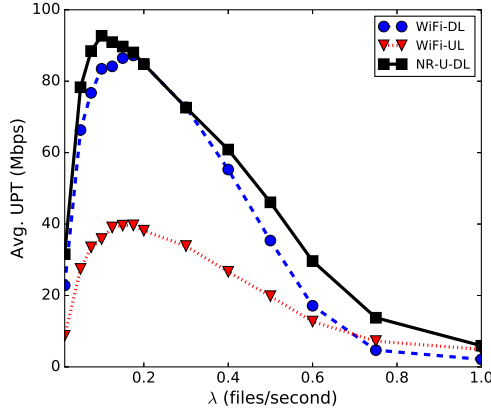
Fig. 13. Average UPT vs. \lambda (indoor at 5.18 GHz; transmit power: 23 dBm; channel bandwidth: 20 MHz; 3GPP InH path loss model).
