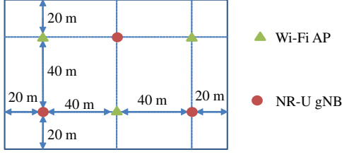
Fig. 8. 3GPP indoor evaluation topology for NR-U/Wi-Fi coexistence [7].
