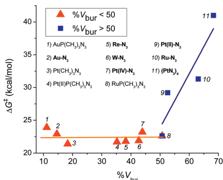
Fig. 8 Plot of calculated \Delta G^\ddagger (kcal mol -1 ) of SPAAC iClick vs. %V bur for all structures investigated in this paper (bolded structures represent experimentally investigated azides). The orange line describes the average \Delta G^\ddagger for azides with a %V bur < 50 ( 23 \pm 1 kcal mol -1 ) and navy line represents the linear relationship between \Delta G^\ddagger of SPAAC iClick and %V bur at %V bur > 50. Passing 50%V bur results in a sharp barrier increase that prevents SPAAC iClick reactivity.
