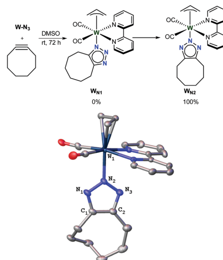
Fig. 2 Synthesis and molecular structure of W N2 with ellipsoids drawn at the 50% probability level and hydrogen atoms removed for clarity. Selected bond distances (Å): W1–N2 2.155(2), N1–N2 1.355(3), N2–N3 1.343(3), N1–C1 1.340(4), N3–C2 1.342(4). Selected bond angles (°): ∠W1–N2–N3 125.85(17), ∠W1–N2–N1 122.20(18), ∠N2–N3–C2 106.20(2), ∠N2–N1–C1 106.10(2).
