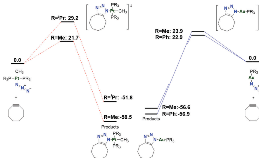
Fig. 6 Computed potential energy surface (units in \text{kcal mol}^{-1} at 298 K and 1 atm; calculated at B3LYP-D0(PCM)/TZ//B3LYP/DZ level of theory) of SPAAC reactions of \text{Pt(II)-N}_3 (red, dashed) and \text{Au-N}_3 (blue, solid). Replacing \text{PPh}_3 with the significantly smaller \text{P(CH}_3)_3 does not affect the barrier height for Au but replacing \text{P}^i\text{Pr}_3 has significant impact on the barrier for the Pt system, suggesting that sterics play an integral part in the SPAAC iClick reactivity of metal azide.
