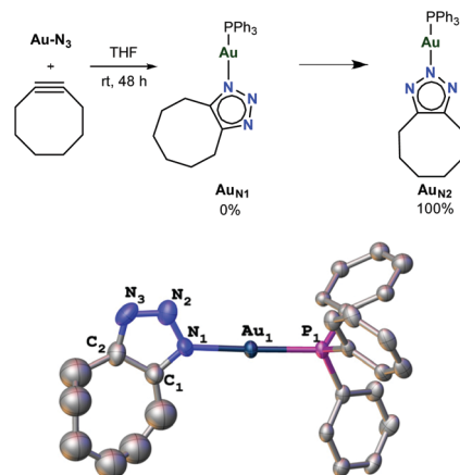
Fig. 1 Synthesis and molecular structure of Au N1 with ellipsoids drawn at the 50% probability level and hydrogen atoms removed for clarity. Selected bond lengths (Å) and angles (°) for Au N1 : Au1–N1 2.061(4), N1–N2 1.299(7), N2–N3 1.258(7), N1–C1 1.334(7), N3–C2 1.389(8), ∠N1–Au1–P1 177.01(13), ∠Au1–N1–N2 119.80(3), ∠Au1–N1–C1 131.00(4), ∠N1–N2–N3 113.60(5).
