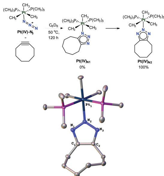
Fig. 7 Synthesis and molecular structure of \text{Pt(IV)}_{\text{N}_2} with ellipsoids drawn at the 50% probability level and hydrogen atoms removed for clarity. Selected bond distances ( \text{\AA} ): Pt1–N2 2.128(2), N1–N2 1.345(3), N2–N3 1.337(3), N3–C2 1.350(3), N1–C1 1.352(3). Selected bond angles ( ^\circ ): \angle\text{Pt1-N2-N3} 123.92(16), \angle\text{Pt1-N2-N1} 122.09(16), \angle\text{N2-N1-C1} 105.20(2), \angle\text{N2-N3-C2} 105.50(2).
