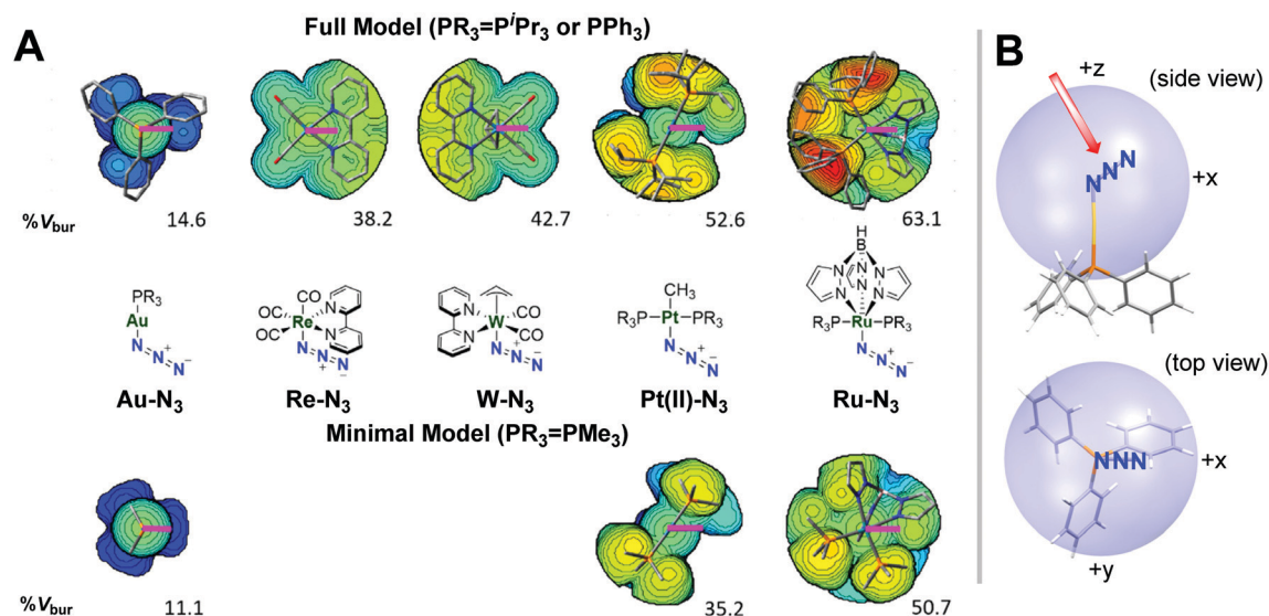
Fig. 5 (A) Topographic maps of the steric hindrance around the azide N1 where cycloaddition occurs (azide centered to right and colored pink for emphasis; blue to red represents increasing steric bulk). Metal azides ordered by increasing %V bur . Top row realistic models, bottom row, minimal models for complex Au-N 3 , Pt(II)-N 3 , and Ru-N 3 (phosphine ligands replaced with P(CH 3 ) 3 ). (B) Orientation of the coordinate system (z-axis: M-N1 bond, xz plane define by M-N1-N2) and location of the scanning sphere (5 Å) on the example of Au-N 3 ; red arrow indicates approach vector of the cyclooctyne.
