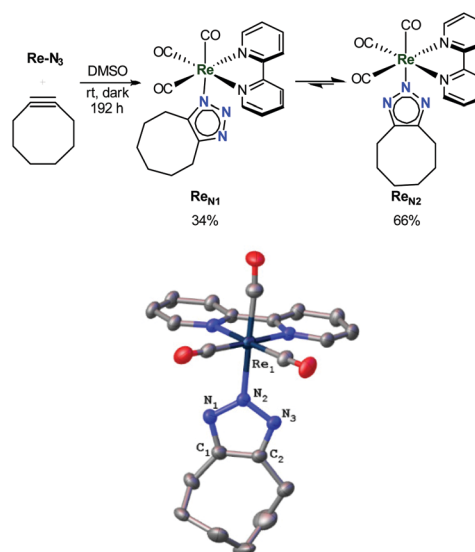
Fig. 3 Synthesis and molecular structure of Re N2 with ellipsoids drawn at the 50% probability level and hydrogen atoms removed for clarity. Selected bond distances (Å): Re1–N2 2.150(2), N1–N2 1.337(3), N2–N3 1.345(3), N3–C2 1.343(3), N1–C1 1.351(4). Selected bond angles (°): ∠Re1–N2–N3 122.88(16), ∠Re1–N2–N1 124.61(17), ∠N2–N1–C1 105.70(2), ∠N2–N3–C2 105.60(2).
