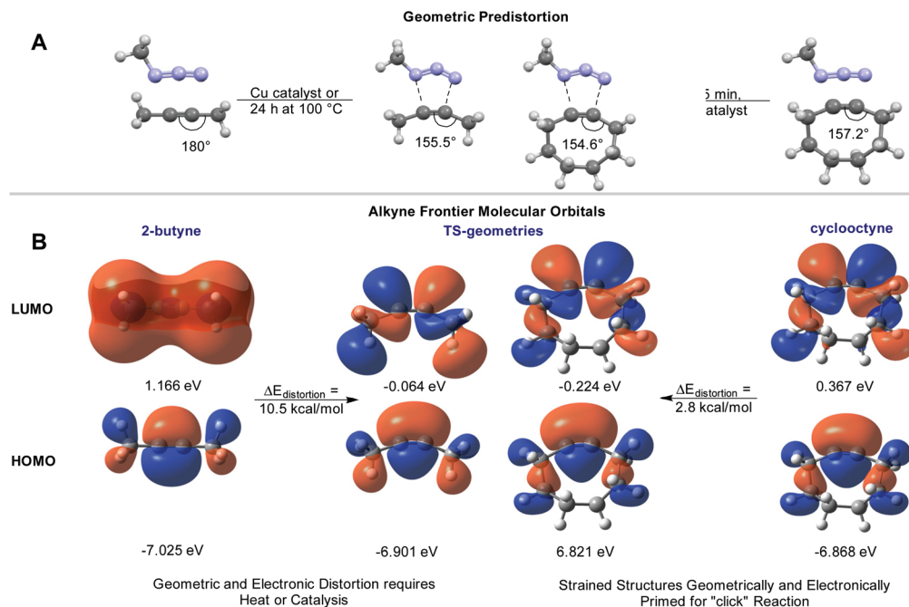
Fig. 4 (A) SPAAC reactions are accelerated due to electronic and geometric predistortion. C–C–C bond angles in cyclooctyne are already at TS state geometry while 2-butyne requires a \sim 25^\circ change. (B) FMO orbitals of cyclooctyne are already primed and the correct LUMO symmetry for 2-butyne is only attained by significant distortion. FMO pictures generated from B3LYP-D0(PCM)/TZ single point energy calculations using GaussView 6, isovalue 0.02. 97
