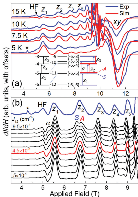
Fig. 10 (a) Experimental (Exp) and simulated (Sim) powder HFEPR spectra of 3.3py-H 2 O at a frequency of 270 GHz, plotted as dI/dH ( I = transmitted intensity) for temperatures in the range from 5 to 15 K. The resonances labeled z_1 to z_4 correspond to the parallel ( z -) components of the powder pattern, xy correspond to the perpendicular components, and HF is a half field transition (see main text for explanation); the feature labeled with an asterisk (*) corresponds to a known O 2 impurity in the sample holder. The inset schematically depicts the lowest lying energy levels appropriate to the parallel resonances. On the left are the uncoupled states associated with each individual S = 6 Mn 3 SMM, labeled according to m_S value, with the m_{S1}, m_{S2} transitions corresponding to resonances z_1 to z_3 labeled. The middle panel shows the levels associated with the uncoupled dimer, labeled according to |m_{S1}, m_{S2}\rangle ; as can be seen, the new states are generated simply by exciting one of the spins, thereby translating (dashed lines) the overall energy of the dimer accordingly. The right panel depicts the fully coupled energy levels, labeled according to |m_{S2}, m_{S1}\rangle , where the blue and red states respectively correspond to the symmetric ( S ) and antisymmetric ( A ) combinations of |m_{S1}, m_{S2}\rangle and |m_{S2}, m_{S1}\rangle . (b) Simulations of the 10 K spectrum as a function of the exchange coupling parameter, J_{12} (in steps of 10^{-3} \text{ cm}^{-1} , see legend). The linewidth is reduced from the best simulations in (a) so that it is possible to resolve additional resonances that emerge due to the exchange coupling, i.e., \alpha and the S and A z_2 resonances. The red simulated spectrum corresponds to the value of J_{12} deduced from magnetic hysteresis experiments and the value used for the simulations in (a).
