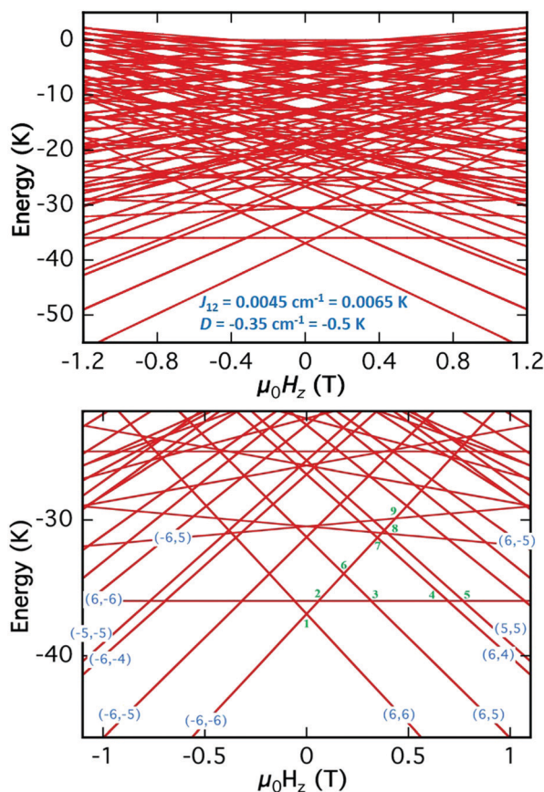
Fig. 8 (Top) Spin state energies vs. applied dc field plot for 3.3\text{py} \cdot 12\text{CH}_2\text{Cl}_2 constructed with J = +4.5 \times 10^{-3} \text{ cm}^{-1} ( \hat{H} = -2J_{12}\hat{S}_1\hat{S}_2 convention) and D = -0.35 \text{ cm}^{-1} to simulate the positions of the avoided level crossings that lead to the experimentally observed QTM step positions in the hysteresis loops of Fig. 6. (Bottom) Expansion showing only the lower energy spin states populated at very low temperature, and the avoided level crossings relevant to the hysteresis loops in Fig. 6 when the field is swept from -1.2 \text{ T} to +1.2 \text{ T} . The green numbers 1 to 9 are the crossings listed in Table 3. Spin states are labelled in blue as (m_{S1}, m_{S2}) for the two \text{Mn}_3 units. See the text for the discussion of the avoided level crossings leading to the observed QTM steps in Fig. 6.
