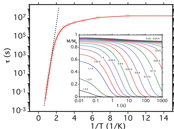
Fig. 7 Relaxation time ( \tau ) vs. 1/T plot for a single crystal of 3\cdot 3\text{py}\cdot 12\text{CH}_2\text{Cl}_2 obtained from the dc magnetization decay vs. time data in zero applied field at the indicated temperatures shown in the inset. The dashed line is the fit of the thermally-activated region to the Arrhenius equation. See the text for the fit parameters.
