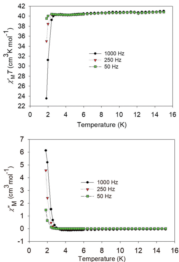
Fig. 5 Plots of the (top) in-phase ( \chi'_{M_r} , as \chi'_M T ) and (bottom) out-of-phase ( \chi''_M ) ac susceptibility data vs. T for 3 \cdot 6\text{H}_2\text{O} in a 3.5 G field at the indicated oscillation frequencies.
