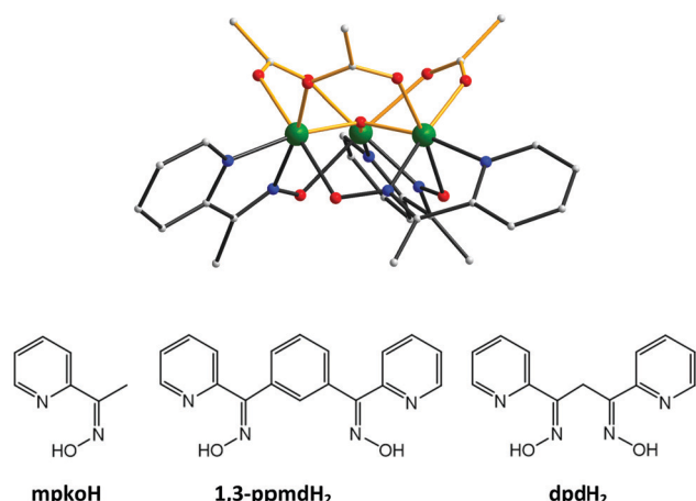
Fig. 1 (top) Structure of the cation of monomer 2 viewed along the \text{Mn}_3 plane showing the tripodal arrangement of the three acetate and three mpko − groups. Colour code: Mn, green; N, blue; O, red; C, gray. (bottom) Structures of mpkoH, 1,3-ppmdH 2 and dpdH 2 .
