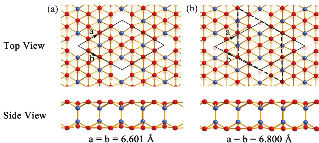
Fig. 6 Top and side views of (a) the eclipsed B_{30} bilayer borophene (A–A packing) 34 and (b) staggered B_{30} bilayer borophene (A–B packing) based on the structural motif of the D_{2h} B_{48} , with the optimized lattice parameters ( a and b ) given at the PBE level. The inward-buckled atoms forming the interlayer B–B \sigma -bonds are highlighted in blue.
