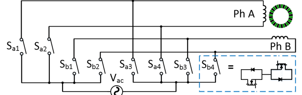
Fig. 2: Matrix converter for single-phase input two-phase output.
