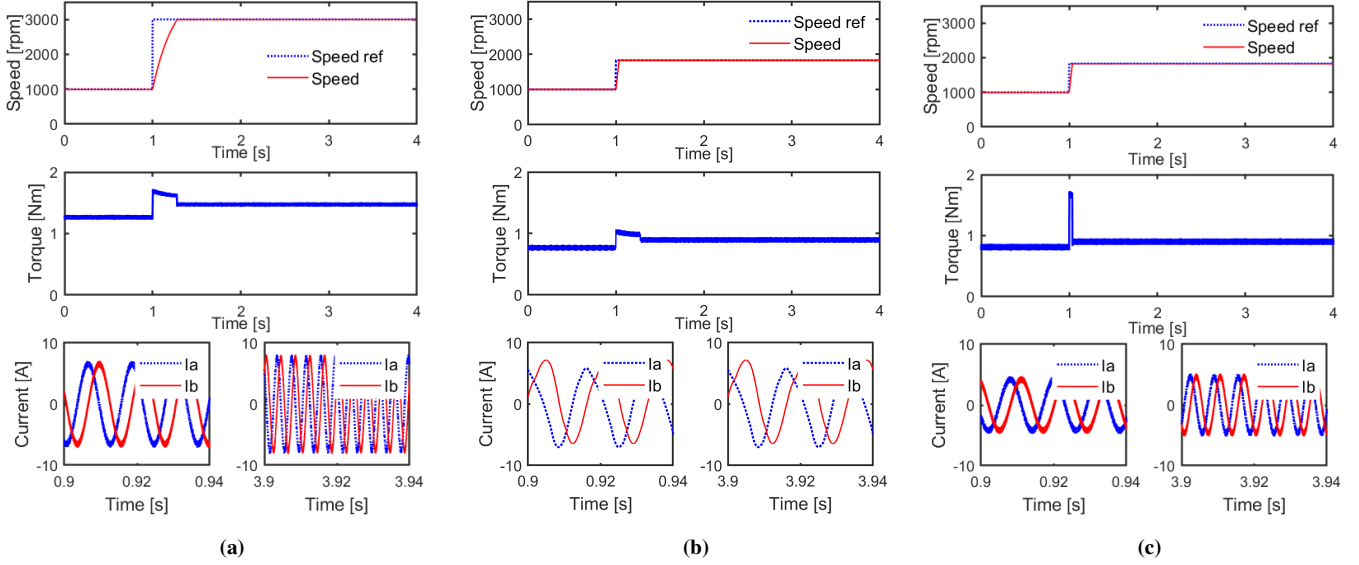
Fig. 8: Simulation results, including the motor speed, estimated electromagnetic torque, and phase currents of closed-loop speed control for a two-phase axial flux PM motor drives in response to the reference speed step change from 1000rpm to maximum operating speed, (a) a conventional single-phase to two-phase back-to-back converter, (b) a single-phase to two-phase matrix converter, and (c) the proposed integrated ac/ac converter.
