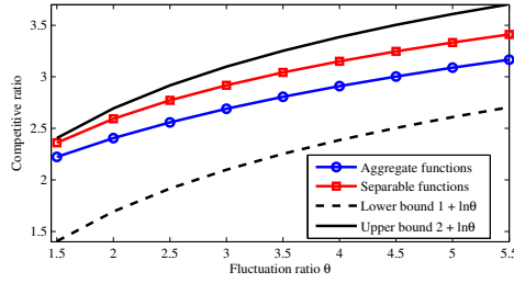
Fig. 1. Competitive ratios of OTA_\phi for FOMKP with aggregate and separable functions.
