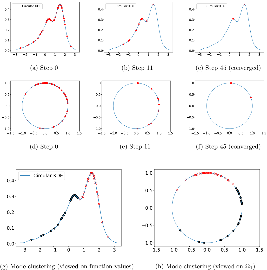
Figure 5: Directional mean shift algorithm performed on simulated data on \Omega_1 . Panel (a)-(c) : Outcomes under different iterations of the algorithm. Panel (d)-(f) : Corresponding locations of points in panels (a)-(c) on a unit circle. Panel (g) and (h) : Visualization of the affiliations of data points after mode clustering.
