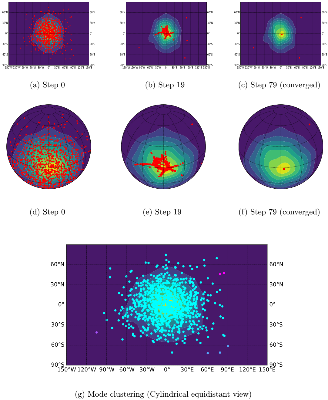
Figure 10: Directional mean shift algorithm performed on simulated data with one mode on \Omega_2 . The analysis is displayed similar to Figure 6. Panel (a)-(c) : Outcomes under different iterations of the algorithm displayed in a cylindrical equidistant view. Panel (d)-(f) : Corresponding locations of points in panels (a-c) in an orthographic view. Panel (g) : Clustering result in a cylindrical equidistant view.
