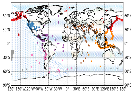
(h) Mode clustering on the world map
