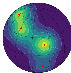
(f) Step 82 (converged)
