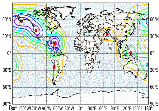
(g) Local modes and contour lines on the world map
