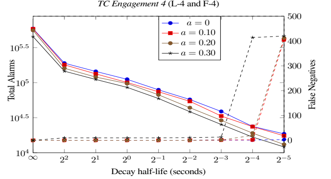
Fig. 5: Total number of alarms and false negatives on TC Engagement 3 and Engagement 4 datasets using different attenuation and decay rates. The scale for total number of alarms is on the left, while the false negative scale is on the right. The total number of true positives are 126 and 425. The total number of alarms without attenuation and decay are 1.69 million and 0.59 million respectively, and they reduce by 10x with tag attenuation and decay.
