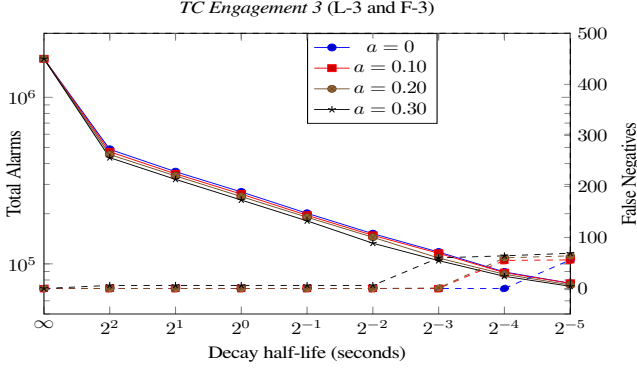
Fig. 5: Total number of alarms and false negatives on TC Engagement 3 and Engagement 4 datasets using different attenuation and decay rates. The scale for total number of alarms is on the left, while the false negative scale is on the right. The total number of true positives are 126 and 425. The total number of alarms without attenuation and decay are 1.69 million and 0.59 million respectively, and they reduce by 10x with tag attenuation and decay.
