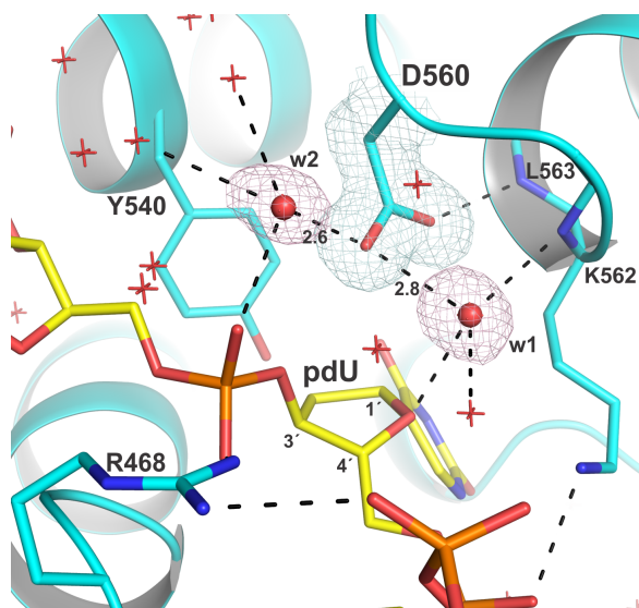
Figure 3. Interactions involving the conserved Asp (D560) in our structure of the MBD4 enzyme-substrate complex with pdU. The 2F_o - F_c electron density map, contoured at 1.0 \sigma , is shown for D560 and two water molecules that contact it, shown as red spheres (w1, w2). The distance of these waters from C1' of pdU is 3.6 Å (w1) and 5.6 Å (w2).
