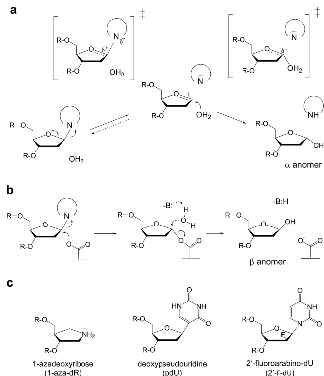
Figure 1. Potential mechanisms for N -glycosyl bond hydrolysis and analogues used in the studies. (a) A direct-displacement reaction following a stepwise ( S_N1 ) mechanism includes an oxacarbenium ion intermediate and two transition states (TS). The AP product exhibits inversion of configuration at the anomeric center ( \alpha -anomer). (b) A double-displacement reaction whereby a carboxylate (Asp or Glu) forms a glycosyl-enzyme intermediate that is hydrolyzed via general base catalysis, giving retention of configuration ( \beta -anomer). (c) Structure of 1-azadeoxyribose and of two deoxyuridine analogues.
