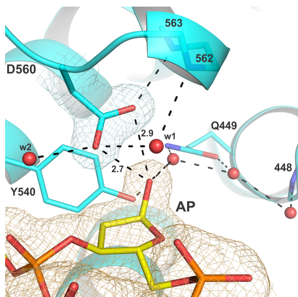
Figure 5. New structure of the MBD4 enzyme-product complex with a focus on the abasic sugar and D560. The 2F_o-F_c electron density map, at 1.0 \sigma , is shown for D560 and DNA.
