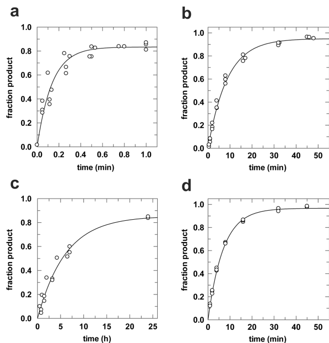
Figure 4. Activity of MBD4 or D560G-MBD4 determined by single turnover kinetics experiments. (a) MBD4 excises 5-CF 3 -uracil or trifluorothymine (T F3 ) from a G·T F3 pair with a rate constant of k_{\text{obs}} = 7.3 \pm 0.8 \text{ min}^{-1} . (b) MBD4 excises T from a G·T pair with a rate constant of k_{\text{obs}} = 0.11 \pm 0.01 \text{ min}^{-1} . (c) D560G-MBD4 excises T F3 from a G·T F3 substrate with a rate constant of k_{\text{obs}} = 0.0027 \pm 0.0003 \text{ min}^{-1} . (d) MBD4 excises T from a G·T pair with a rate constant of k_{\text{obs}} = 0.14 \pm 0.01 \text{ min}^{-1} in reaction buffer for which NaCl is replaced with KCl. Experiments were collected with 0.5 \mu\text{M} substrate and 5.0 \mu\text{M} enzyme, at 23 °C.
