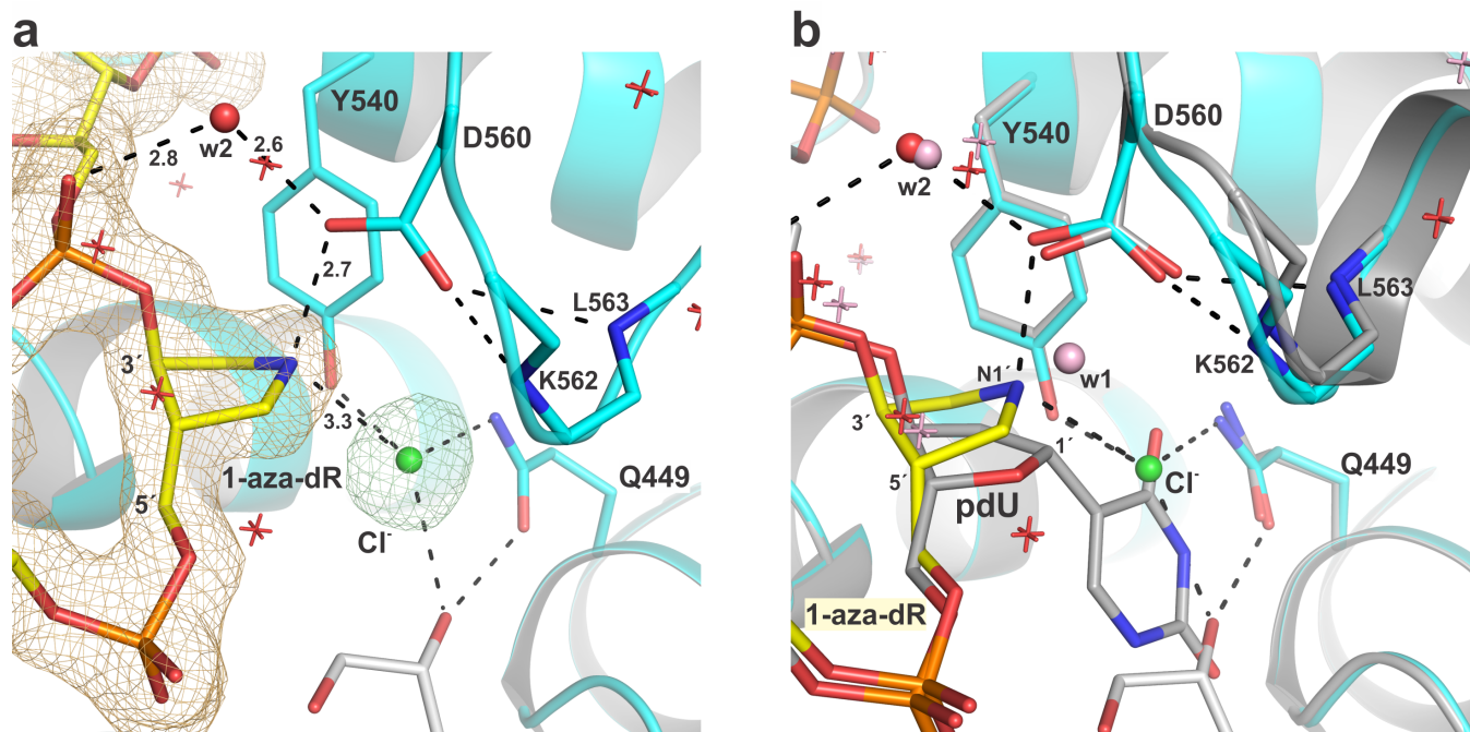
Figure 6. Structure of DNA-bound MBD4 with 1-aza-dR flipped into its active site, a mimic of the putative E·I complex (PDB ID: 7KZG). (a) Closeup view of active site showing interactions involving 1-aza-dR and D560. The water molecule (w2) contacting D560 and a backbone phosphate is shown as a red sphere and other waters are red crosses. The 2F_o - F_c electron density map (at 1.0 \sigma ) is shown for DNA containing 1-aza-dR and the Cl ion (green). A solvent molecule is shown in white (modeled as glycerol but electron density suggests possibility for partial occupancy by water molecules). (b) Structural alignment of our models for the E·I complex (1-aza-dR) and the E·S complex (pdU). The electrostatic interactions and coloring for the E·I complex are as shown in panel 5a; coloring for the E·S complex is grey for MBD4 and DNA and pink for water molecules. Two water molecules (w1, w2) contact D560 in the E·S complex while only one of these (w2) does so in the E·I complex.
