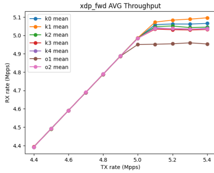
(g) xdp_fwd: Throughput vs. Offered load
