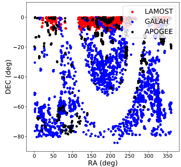
Figure 2. Spatial location of stars with SkyMapper photometric metallicities that also have high-quality metallicities (see Section 3.1 for a description) from LAMOST DR6 (red), GALAH DR3 (blue), and APOGEE DR16 (black).
