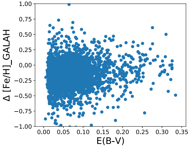
Figure 5. Residuals of the final photometric metallicities with respect to metallicities from GALAH DR3 shown as a function of the reddening values from Schlegel et al. (1998). No strong systematics appear as a function of reddening value out to E(B - V) \sim 0.35 , beyond an offset with metallicities in GALAH DR3.
