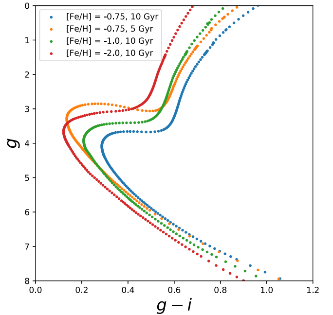
Figure 6. Dartmouth isochrones of [\text{Fe}/\text{H}] = -0.75 , -1.0 , and -2.0 plotted with the SkyMapper g - i color and absolute g magnitude. We flag stars in our sample that have absolute SkyMapper g > 5.0 or that are redward of the [\text{Fe}/\text{H}] = -0.5 , 10 Gyr isochrone as plausible main-sequence or metal-rich contaminants in our sample (see Section 2.4). We show the [\text{Fe}/\text{H}] = -0.75 isochrone with two ages for illustrative purposes.
