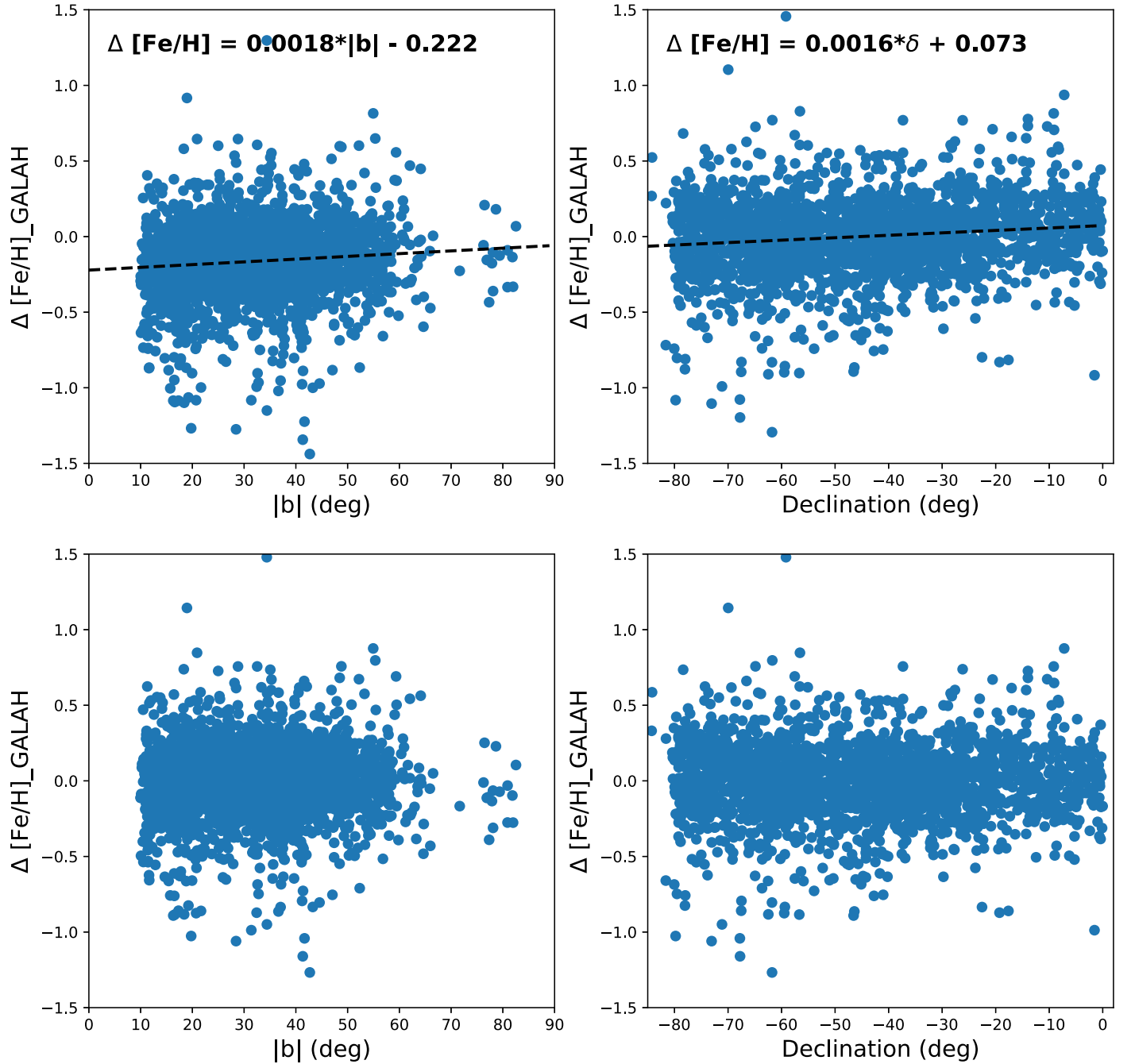
Figure 3. Top left: residuals of the initial photometric metallicities derived in Section 2.2 with respect to metallicities of stars in GALAH DR3 as a function of Galactic latitude. A line is fit to the residuals and the trend is subtracted from the initial photometric metallicity determination to account for the spatial variation of the metallicity. Top right: same as the top left, but shown as a function of decl. Bottom left: Residuals of the photometric metallicities after removing the trend as a function of Galactic latitude. No further trends are apparent. Bottom right: same as the bottom left, but shown as a function of decl.
