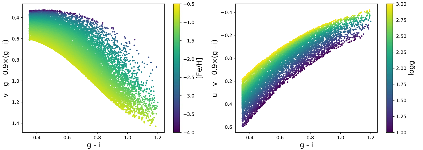
Figure 1. Left: metallicity-sensitive color-color plot that was used to derive photometric metallicities (see Section 2.2), where each point corresponds to a star in SkyMapper DR2. Right: surface-gravity-sensitive color-color plot, where each point also corresponds to a star in SkyMapper DR2.
