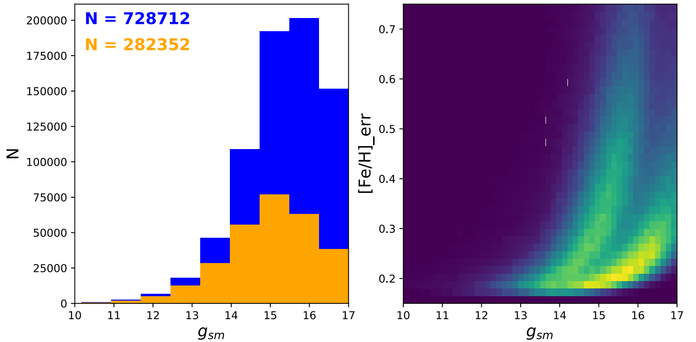
Figure 7. Left: histogram of the magnitudes of all stars in our catalog (blue) and those passing the flags in Section 2.4 (orange). Right: uncertainties on the photometric metallicities of the stars in our sample as a function of magnitude.
