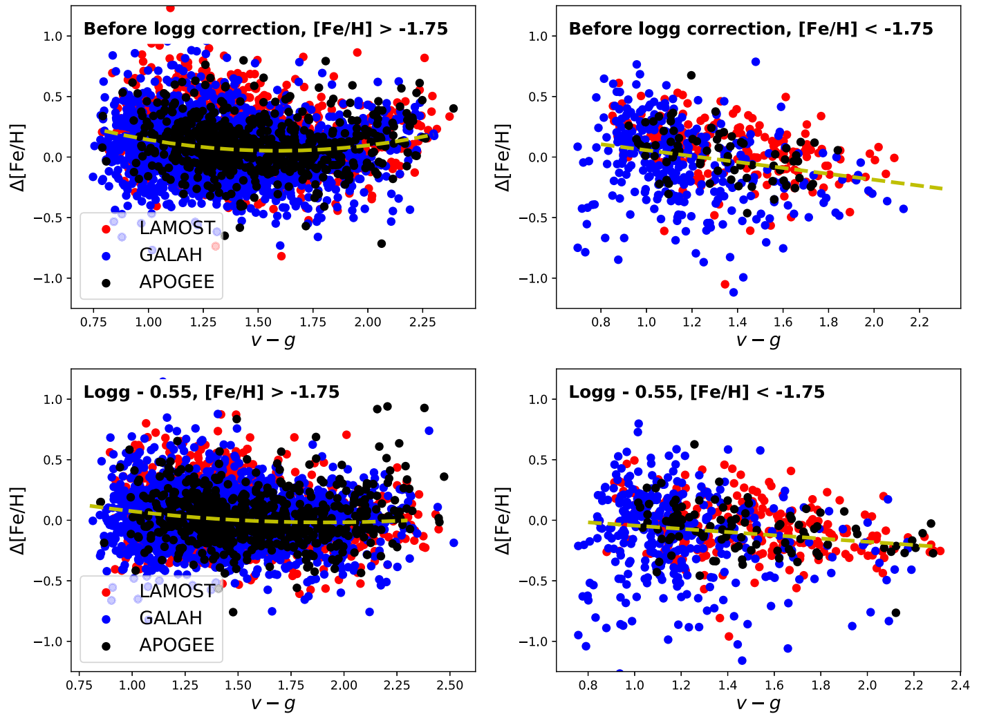
Figure 4. Top left: residuals of our initial photometric metallicities derived in Section 2.2 with respect to high-quality (see Section 3.1 for a full description) metallicities of stars in LAMOST DR6 (red), GALAH DR3 (blue), and APOGEE DR16 (black) as a function of the v - g color for stars with photometric metallicities [\text{Fe}/\text{H}] > -1.75 . A clear quadratic trend is apparent in the residuals. Note that the residuals with respect to each survey have been slightly adjusted to account for zero-point offsets in metallicities. Top right: same as left, but residuals are shown for stars with photometric [\text{Fe}/\text{H}] < -1.75 for which a slightly different trend is apparent. Bottom left and right: same as top panels, but using photometric metallicities that were calculated after decreasing the photometric \log g by 0.55 dex to bring our surface gravity scale in agreement with that in Ezzeddine et al. (2020) and X. Ou et al. (in preparation). Only negligible trends in the residual metallicities exist after the surface gravity correction.
