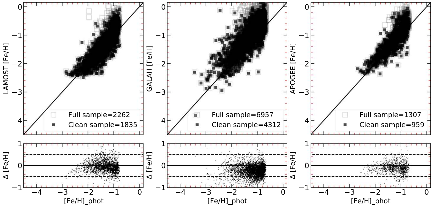
Figure 8. Our SkyMapper photometric metallicities, compared to metallicities from LAMOST DR6 (left panels), GALAH DR3 (middle panels), and APOGEE DR16 (right panels) for stars with photometric metallicity uncertainties lower than 0.30 dex. The filled black squares correspond to stars that passed the flags in Section 2.4, and the open squares correspond to the entire sample. The lower panels show the residuals between our photometric metallicities and those presented in the above surveys. Dashed lines indicate \pm 0.50 to guide the eye. The agreement between our metallicities and those presented in these surveys is good, as indicated by the relatively low standard deviation of the residuals in the bottom panel ( \sim 0.25 dex) despite slight offsets with each survey.
