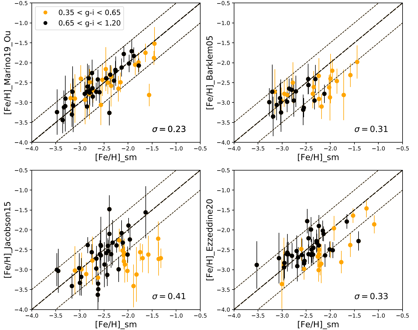
Figure 9. Top left: a comparison between the photometric metallicities of stars presented in our catalog and metallicities from the high-resolution spectroscopy of Marino et al. (2019) and X. Ou et al. (2021, in preparation). Top right: same comparison but with the high-resolution spectroscopy results of Barklem et al. (2005). Bottom right: same comparison but with the high-resolution spectroscopy results of Ezzeddine et al. (2020). Bottom left: same comparison but with the high-resolution spectroscopy results of Jacobson et al. (2015). The black data points correspond to cooler stars in our sample ( g - i > 0.65 ) and orange data points to warmer stars ( g - i < 0.65 ). There is some evidence that our photometric metallicities are biased high with respect to three of the studies when g - i < 0.65 . Lines are drawn at \pm 0.5 dex to guide the eye. The \sigma in each panel corresponds to the standard deviation of the metallicity residuals between our catalog and the corresponding study for stars with g - i > 0.65 .
