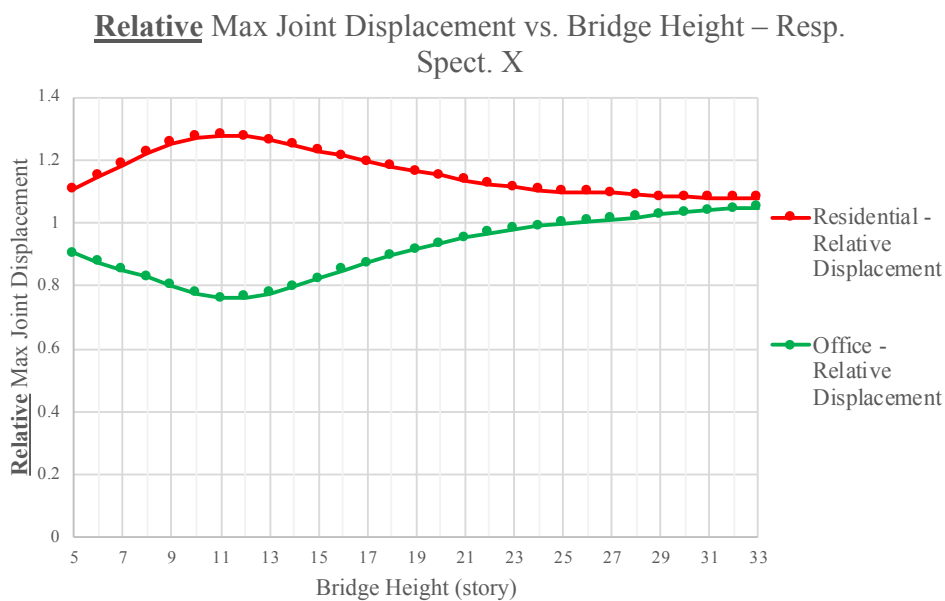
Fig. 7 – Relative Max Joint Displacement vs. Skybridge Height
