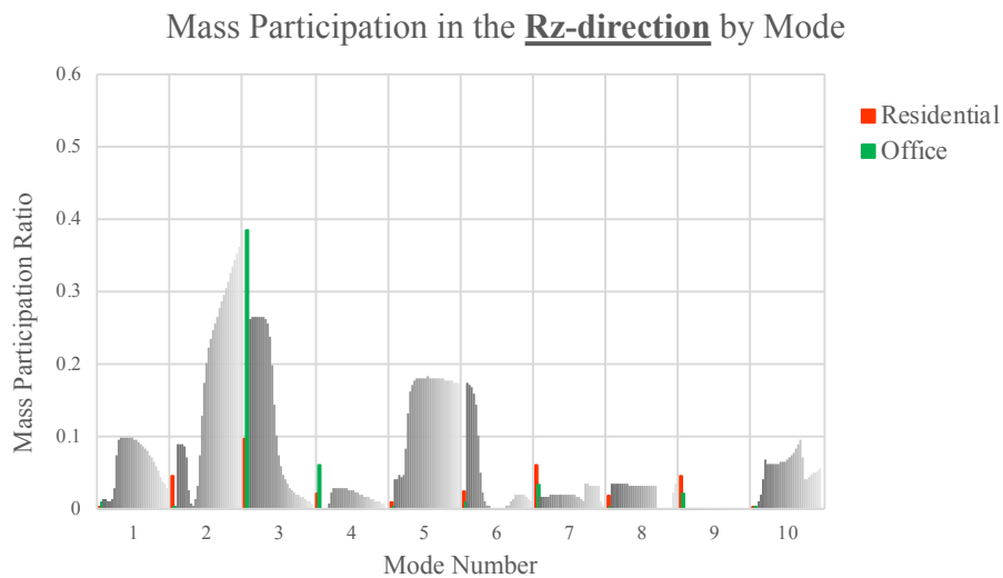
Fig. 6 – MPR in the Rz-direction by Mode
