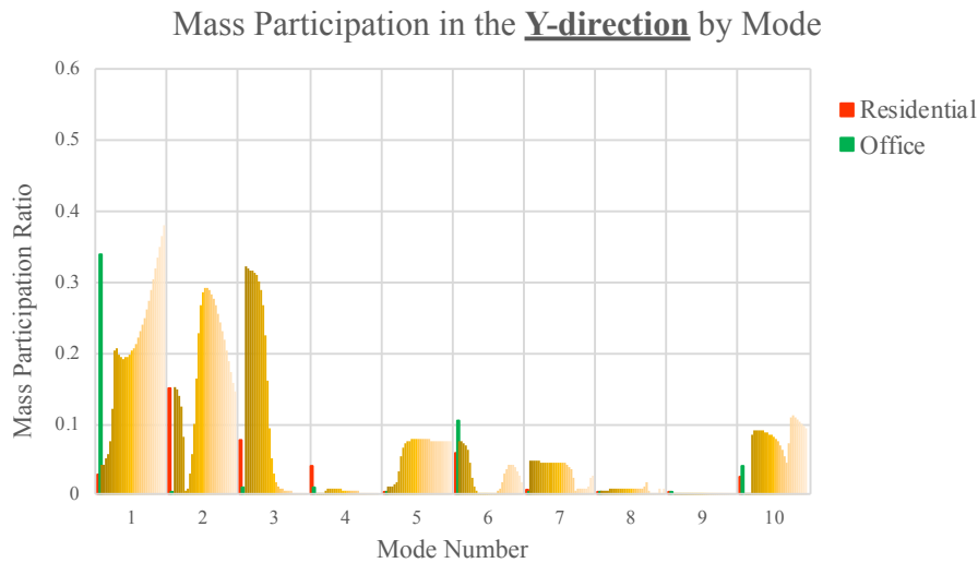
Fig. 5 – MPR in the Y-direction by Mode
