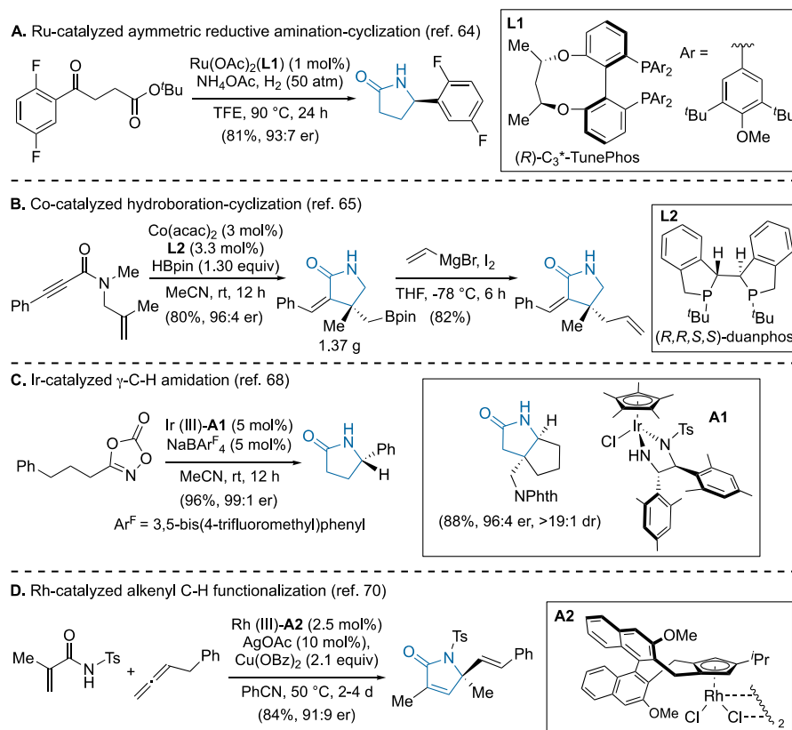
Scheme 2. Enantioselective transition metal-catalyzed \gamma -lactam synthesis
