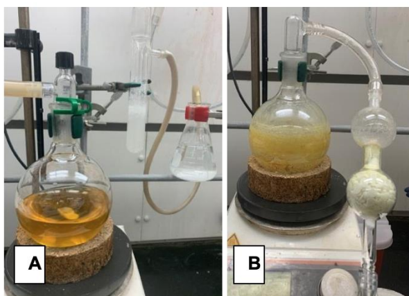
Figure 3. Acid chloride synthesis: A) Reaction set up with mineral oil bubbler and sodium bicarbonate solution in sequence to control and quench exhaust gases. B) Crude acid chloride used in the next reaction after drying on high vacuum with an attached acid scrubber (KOH pellets) (photos provided by submitters).
