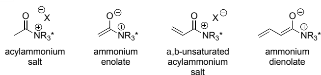
Figure 12. Chiral acylammonium salt intermediates
