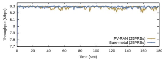
Fig. 6: Throughput for 25 PRBs
