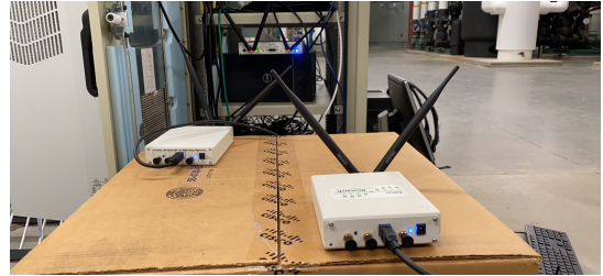
Fig. 5: PV-RAN testbed at ISU Research Park
