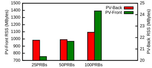
Fig. 10: Resident Set Size (RSS) of Dom0 PV-Back and DomU PV-Front for different channel bandwidths
