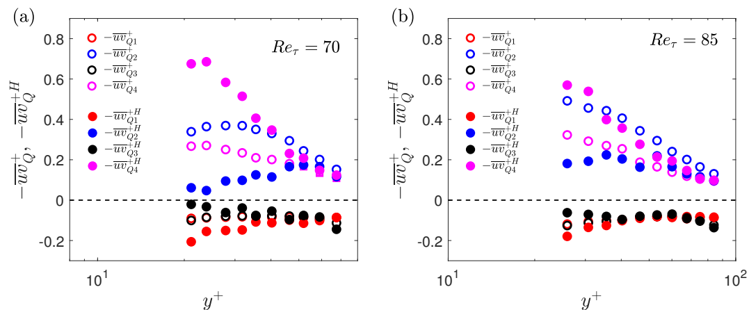
Figure 18. (a) Contribution to -\overline{uv} from different quadrants for the unconditional case and during the high-drag events for (a) Re_\tau = 70 and (b) Re_\tau = 85 . The criteria to detect a high-drag event is \Delta t_{cr}^+ = 200 and \tau_w/\overline{\tau_w} < 0.9 . Thin black dashed line represents a constant value of zero.
