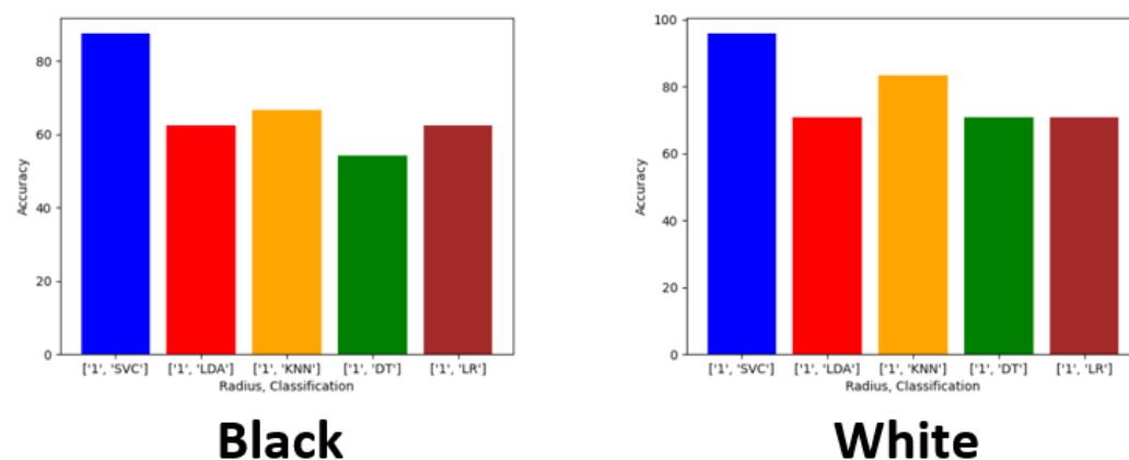
Figure 6. ML accuracies with imbalanced datasets and 11 training images.
