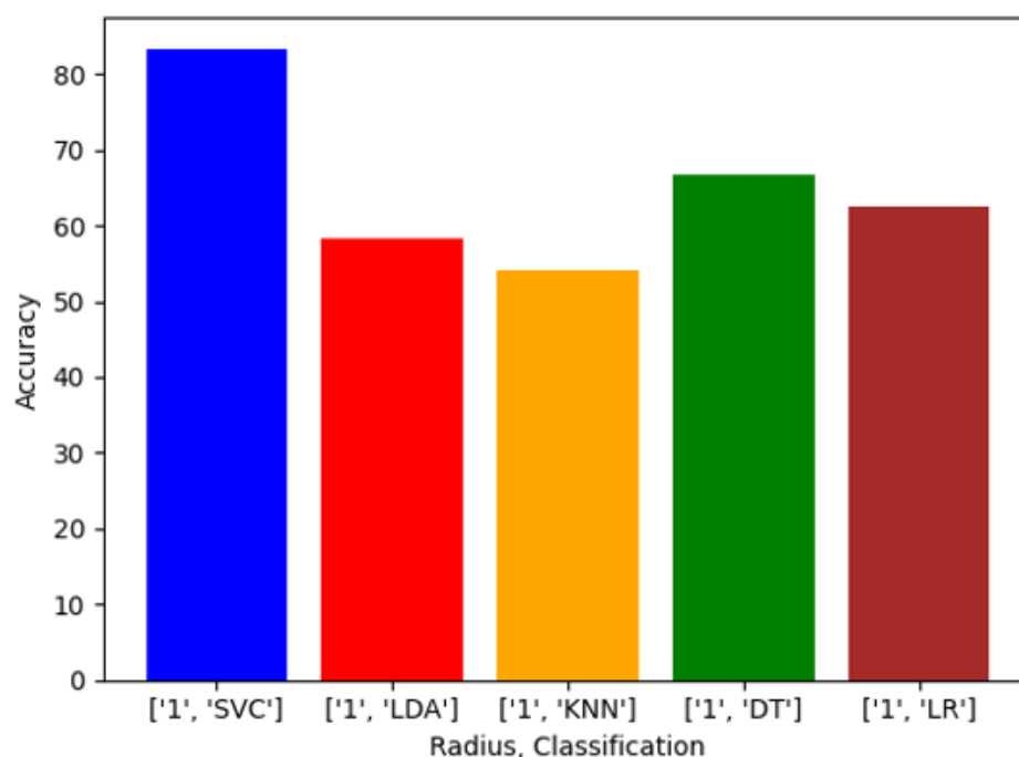
Figure 3. ML accuracies with balanced dataset and 8 training images.
