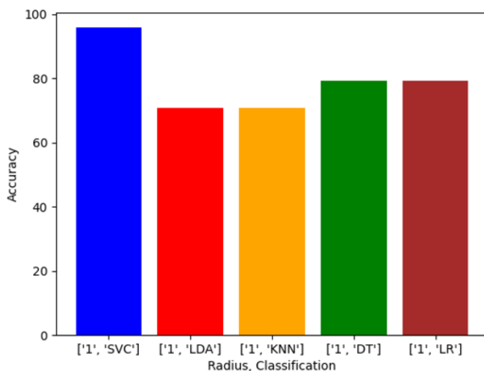
Figure 7. ML accuracies with a balanced dataset and 22 training images.
