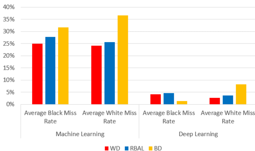
Figure 18. Miss rates for all datasets.
