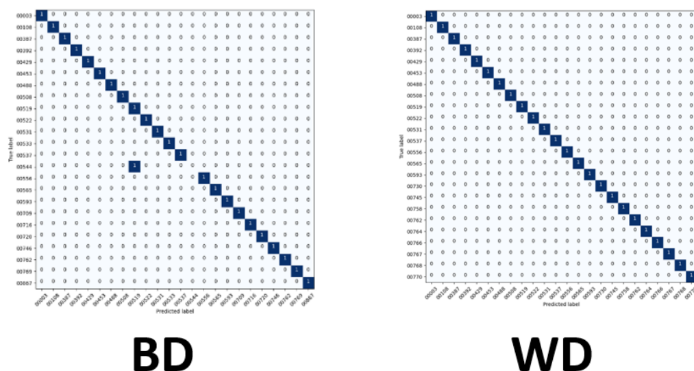
Figure 15. ResNet50 imbalanced confusion matrices using 22 training images.
