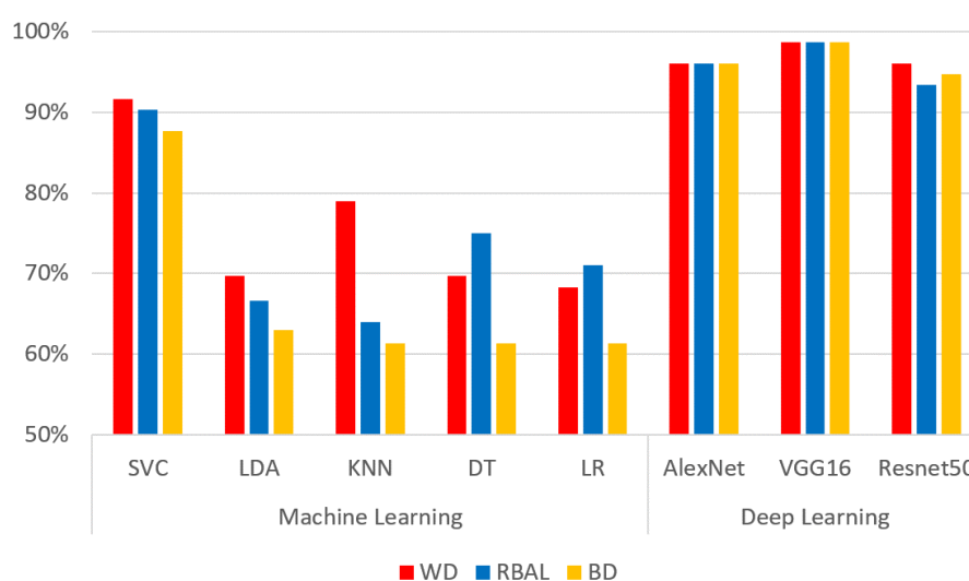
Figure 17. Complete algorithms summary with all datasets.
