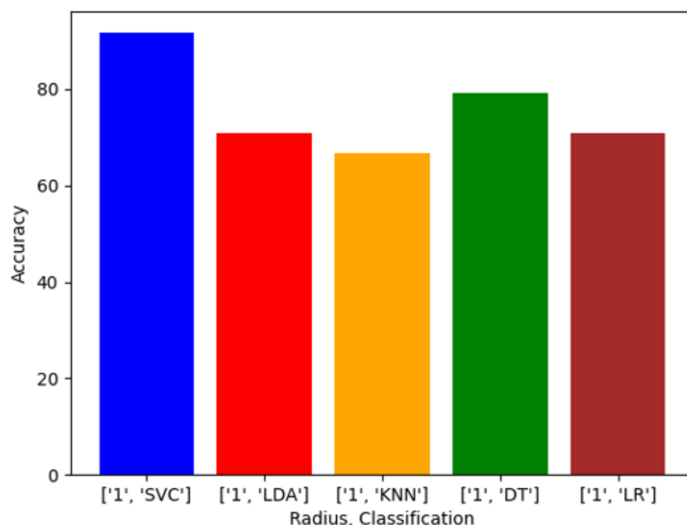
Figure 5. ML accuracies with balanced dataset and 11 training images.
