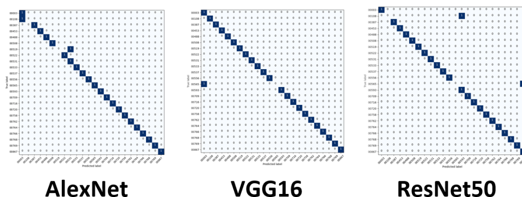
Figure 10. DL confusion matrices using balanced datasets and 8 training images.
