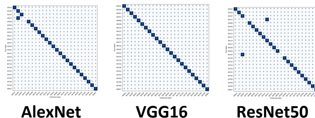
Figure 12. DL confusion matrices using balanced datasets and 11 training images.
