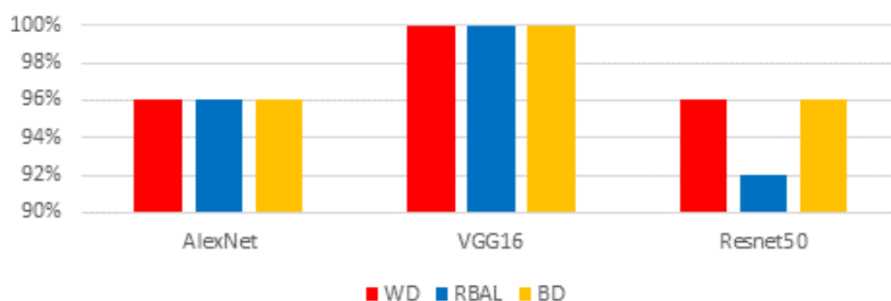
Figure 13. DL accuracies on all datasets using 11 training images.
