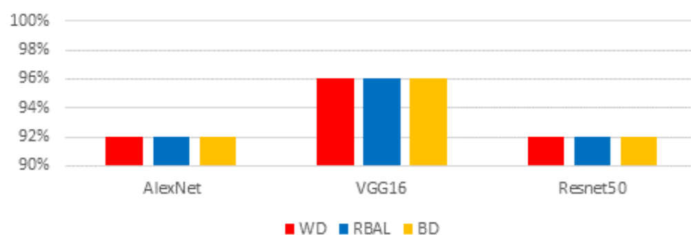
Figure 11. DL accuracies on all datasets using 8 training images.
