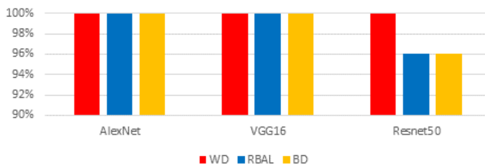
Figure 16. DL accuracies on all datasets using 22 training images.
