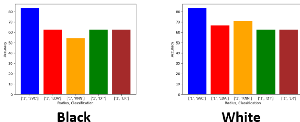
Figure 4. ML accuracies with imbalanced datasets and 8 training images.
