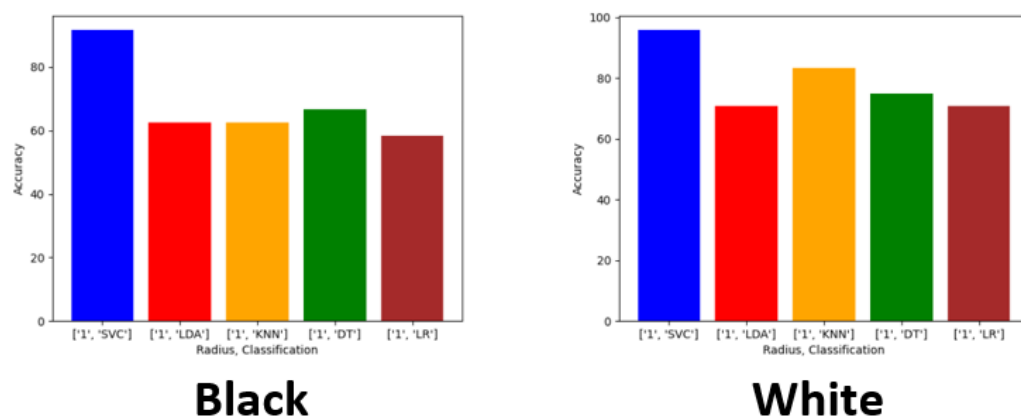
Figure 8. ML accuracies with imbalanced datasets and 22 training images.
