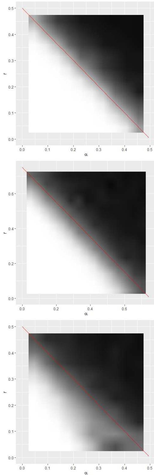
FIG 1. The power of testing procedures in the dense signal setup. (a) shows the power of the conditionally centered magnetization test for \theta = 0.5 , (b) shows the power of the total magnetization test for \theta = 1 (c) shows the power of the conditionally centered magnetization test for \theta = 1.5 . The theoretical detection threshold is drawn in red.
