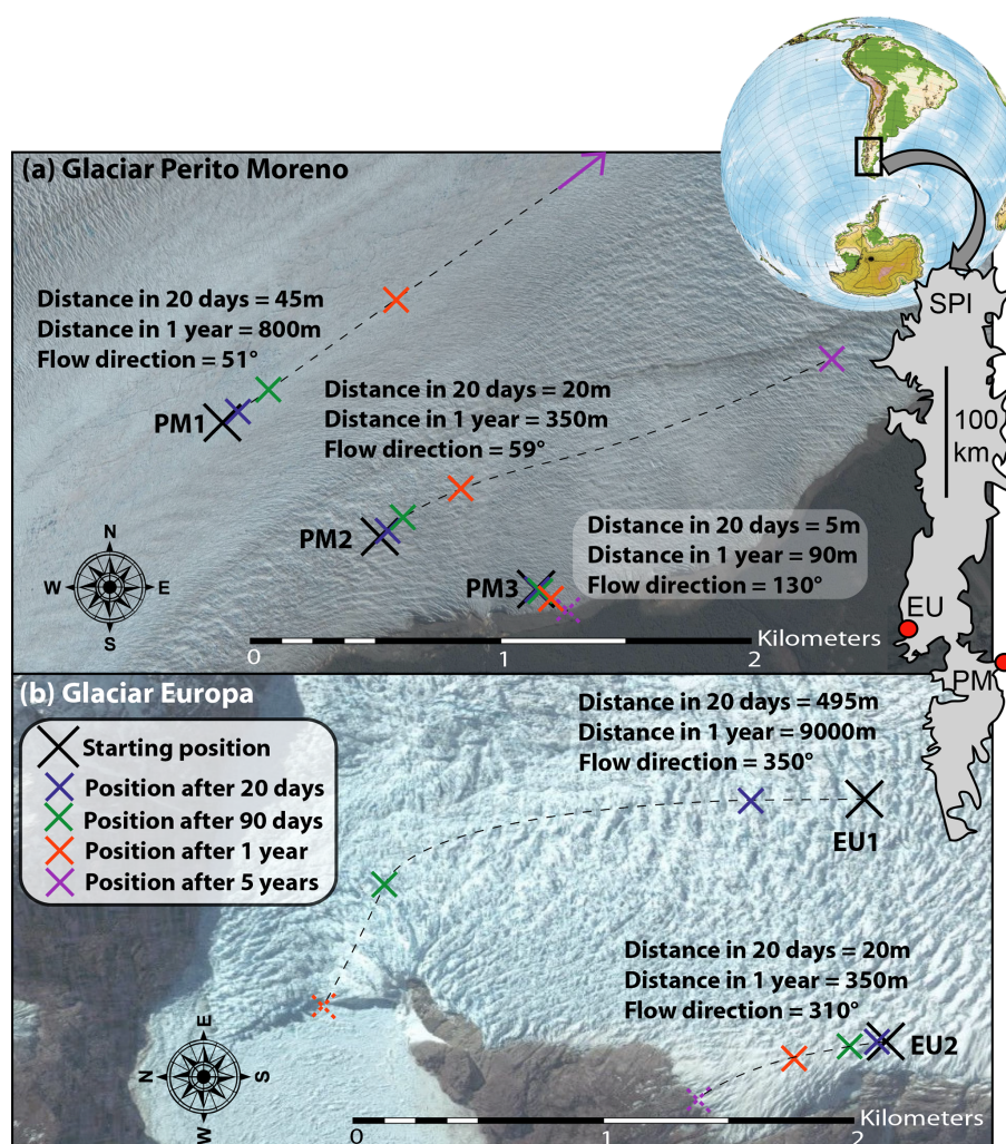
Figure 6. (a) Position of a point on Glaciar Perito Moreno (PM) with the time for three different starting locations within 2 km of the glacier's southern margin. At PM1, ice speeds reach 800 \text{ m yr}^{-1} , and any equipment will be rapidly displaced. At PM3 ice-flow speeds are < 100 \text{ m yr}^{-1} and oriented towards the valley edge. (b) Identical plot for two points on Glaciar Europa (EU). Any equipment installed at EU1 will be displaced several kilometres and lost to calving in less than 6 months. The inset shows an outline of the Southern Patagonian Icefield (SPI) with the locations of the two glaciers. Imagery © Google Earth.
