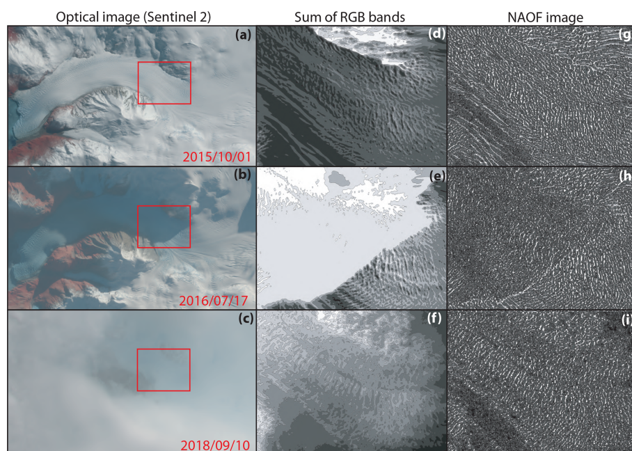
Figure 2. Comparison between raw optical images, band-summed images, and NAOF-filtered images for a clear image (a, d, g), a heavily shadowed image (b, e, h), and a cloudy image (c, f, i) of Amalia glacier, Patagonia ( -50.92^{\circ} S, -73.56^{\circ} W). Note how despite the complexity, the NAOF images recover a clear and easily traceable feature pattern on the surface of the glacier that is suitable for obtaining velocities. The shadow line leaves an artefact in (h) but is a marked improvement on the lack of features in the shaded area in (e). Images from Sentinel-2.
