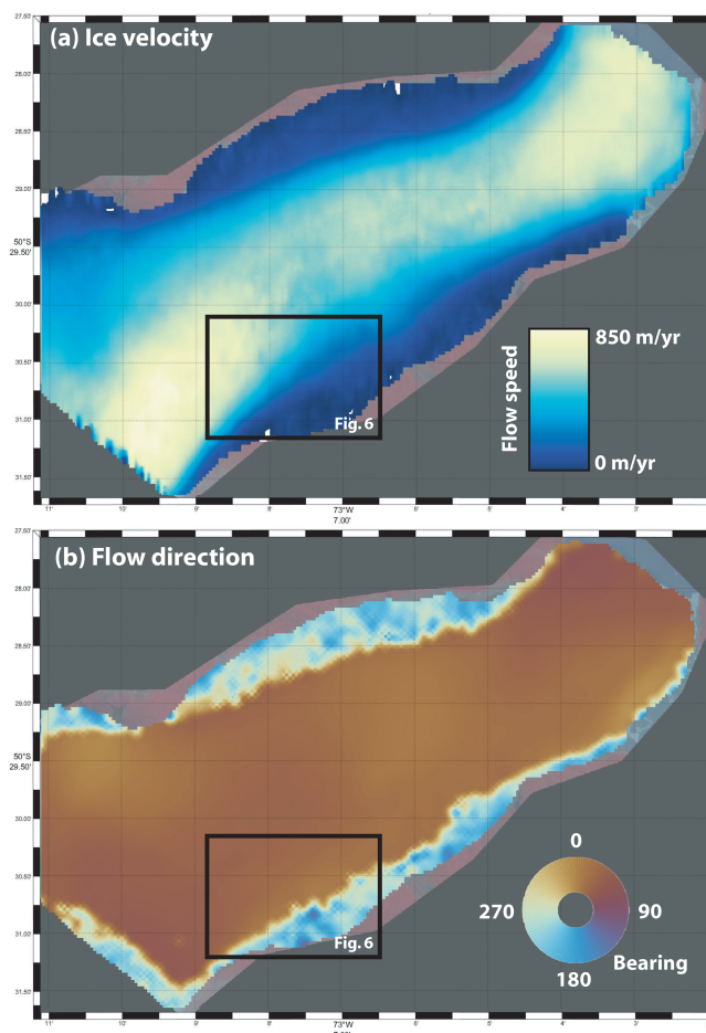
Figure 5. Mean flow velocity ( \text{m yr}^{-1} ) (a) and direction (degrees) (b) of Glacier Perito Moreno, Argentina, for the first 3 months of 2020. Figure panels have been automatically generated from GIV, labels have been added, and the colour bars moved.
