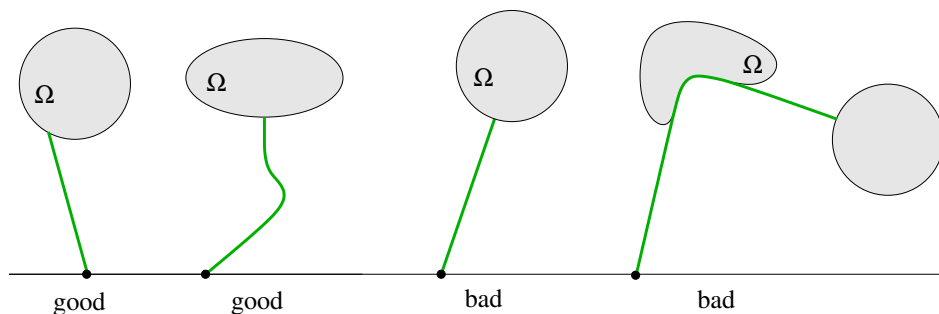
FIGURE 3. For the two initial configurations on the left, the constrained growth equation (8) admits a unique solution. On the other hand, the two configurations on the right satisfy both (26) and (27) in (B). In such cases, the Cauchy problem is ill posed.
