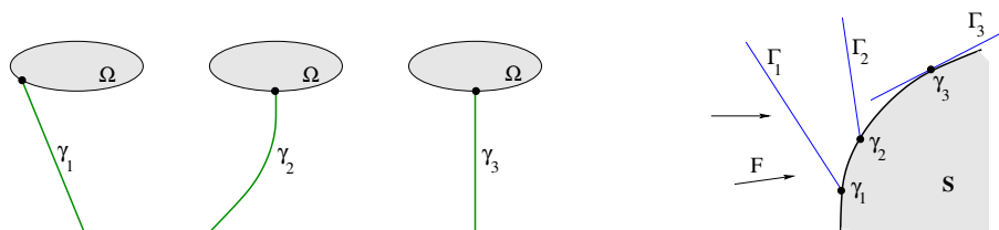
FIGURE 2. Left: three configurations of the stem, relative to the obstacle. Right: in an abstract space, the first two configurations are represented by points \gamma_1, \gamma_2 on the boundary of the admissible set S where the corresponding cones \Gamma_1, \Gamma_2 are transversal. On the other hand, \gamma_3 is a “breakdown configuration”, satisfying all assumptions (26)-(27). Its corresponding cone \Gamma_3 is tangent to the boundary of the set S . Here the shaded region is the complement of S .
