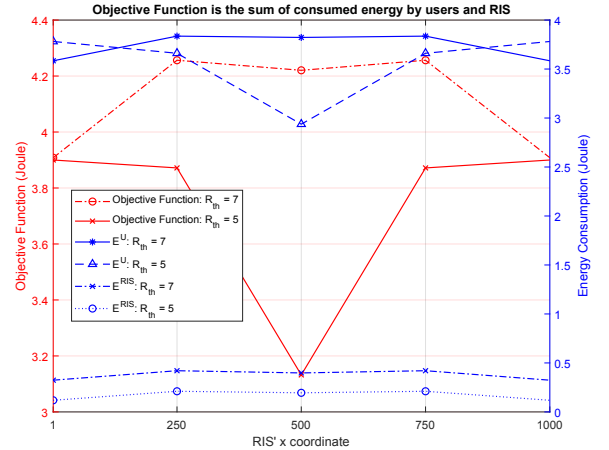
Fig. 3: Sum of energy consumed by the RIS and users vs. different R_{th} values and RIS's locations.
