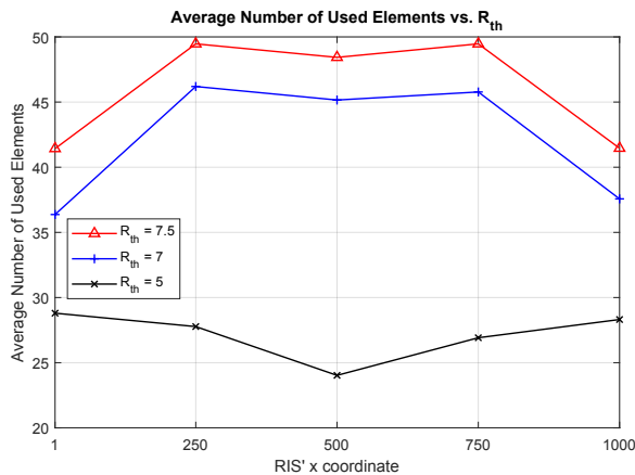
Fig. 5: Average number of used RIS's elements vs. different R_{th} values and RIS's locations.
