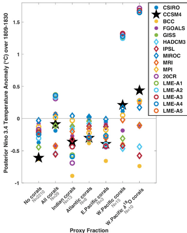
FIG. 6. As in Fig. 4, but considering multiple climate model priors. The 1809–30 average for each prior is plotted with a single data point. The results from CCSM4 in Fig. 4 are illustrated with black stars. Coral-based reconstructions yield a much wider spread of estimated Niño-3.4 behavior, especially corals from the western Pacific.
