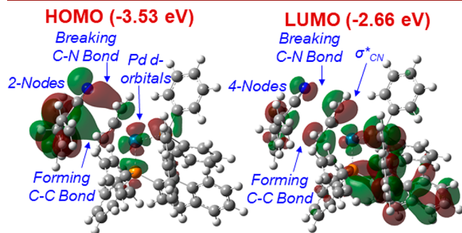
Figure 1. Calculated molecular orbitals for TS-[3,3]-Pd
