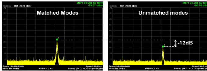
Fig. 11. Measured spectrum of combined IF in Rx mode when modes are matched and unmatched
