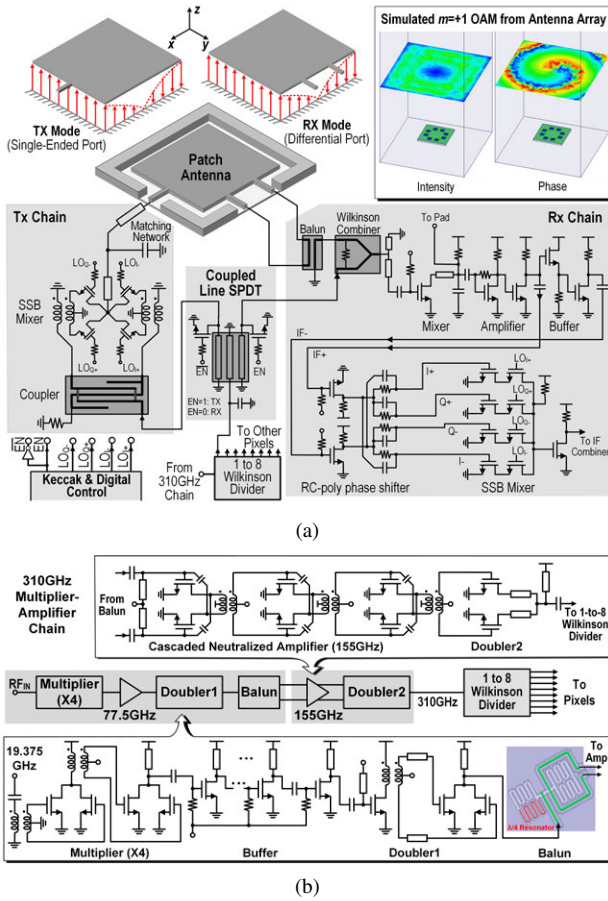
Fig. 3. Schematics of (a) the 310GHz OAM pixel, and (b) the 310GHz multiplier-amplifier chain.
