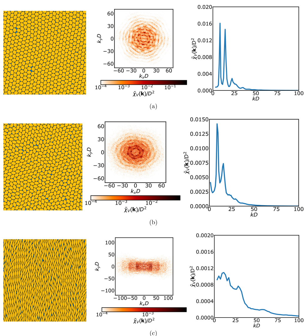
Figure 12. Example representative configurations (left), corresponding two-dimensional (center), and angular averaged spectral densities (right) \tilde{\chi}_V(\mathbf{k})/D^2 vs dimensionless wavenumber kD from lens packings: (a) \alpha = 0.8 lenses compressed using the slow compression schedule, (b) \alpha = 0.666... lenses compressed using the medium compression schedule, and (c) \alpha = 0.2 lenses compressed using the slow compression schedule, where D is the circumradius of the particle.
