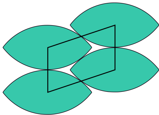
Figure 3. Fundamental basis of the putative densest \alpha = 0.5 lens packing.
