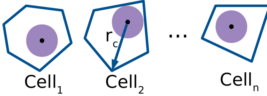
Figure 10: A schematic of Voronoi cells and spherical covering areas that demonstrates that the E_V(r) of a crystalline system decays as a power-law with exponent \gamma = d close to the critical-hole size. A crystal has a finite number of distinct Voronoi cells, and thus there exists a gap between the set of vertices at a distance r_c and the next farthest set of vertices. Thus, we can conclude the proposed behavior through considering the decrease in volume of a small uncovered corner.
