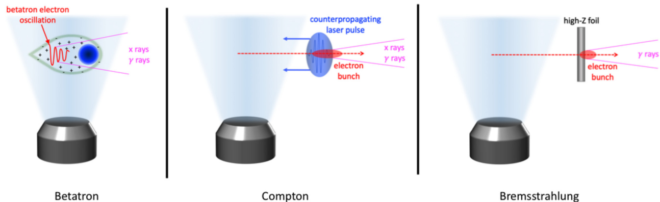
FIG. 7. Principle of betatron, inverse-compton and bremsstrahlung radiation sources. In the first case (left), electrons oscillate in the blow-out cavity of the laser-plasma accelerator and radiate betatron x-rays. For the inverse-compton source (middle), at the exit of the laser-plasma accelerator, electrons radiate IC scattered photons during their oscillations in the field of a counterpropagating laser pulse. Bremsstrahlung radiation (right) can be produced by placing a high-Z foil in the path of the electron beam.
