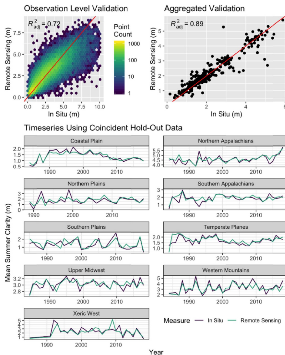
Figure 1. Model validation based on hold-out data not used in model development. Clockwise from the upper left: point based model performance, model performance aggregated by year and region, and regional timeseries of aggregated validation. Note that the time series shown only include hold-out estimates coincident with field measurements used for validation and do not represent the final time series of the study. They are provided to illustrate that the validation captures regional temporal patterns seen in the field data.
