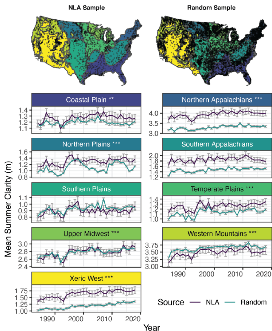
Figure 2. Regional modelled trends in water clarity for the statistically stratified sample of NLA lakes that are Landsat visible and a large random sample of Landsat visible lakes. Trends and their associated confidence intervals represent the mean and standard deviation of values calculated through 1000 iterations of bootstrap sampling of the NLA and random sample lakes respectively. Points on maps represent individual lakes included in the sample. Asterisks indicate significance levels of trends determined by Thiel–Sen slopes at 90% (*), 95% (**), and 99% (***) confidence levels for the NLA sample of lakes.
