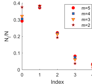
Fig. 4. The index distribution for different m where H = 1 , d_x = 2 , d_y = 2 , and \Lambda_{\max} = 1 .
