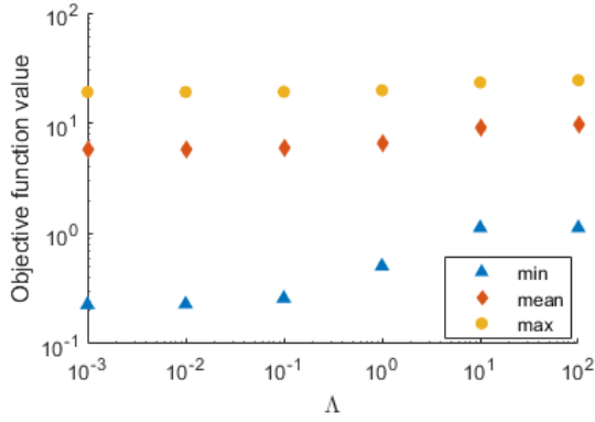
Fig. 5. The minimum, mean, and maximum of global minimum loss function value at real solutions of 1000 samples with different \Lambda_{\max} . The other parameters are H = 1 , m = 5 , and d_1 = d_x = d_y = 2 .
