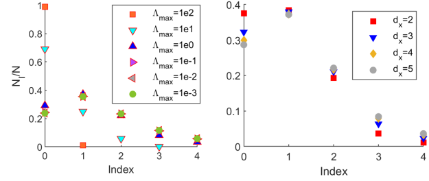
Fig. 3. The index distribution for different d_x and \Lambda_{\max} . For the left plot, H = 1 , m = 5 , d_x = d_y = d_1 = 2 , and \Lambda \in [0, \Lambda_{\max}] . For the right plot, H = 1 , m = 2 , d_y = d_1 = 2 , and \Lambda_{\max} = 1 .
