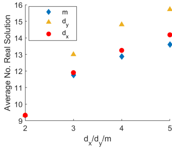
Fig. 2. The mean of \mathcal{N}_R for different value of d_x (circles), d_y (triangles) and m (diamonds) where \Lambda_{\max} = 1 . For circles: H = 1 , m = 2 , and d_y = d_1 = 2 . For triangles: H = 1 , m = 2 , and d_x = d_1 = 2 . For diamonds: H = 1 and d_x = d_y = d_1 = 2 .
