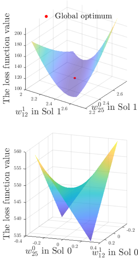
Fig. 6. The loss surfaces near two solutions found by Bertini. The top figure shows the loss surfaces for Solution 1 against variable w_{12}^1 and w_{25}^0 . The bottom figure shows the loss surfaces for zero solution against variable w_{12}^1 and w_{25}^0 .
