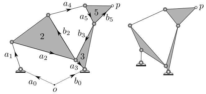
Fig. 4. Watt-1A mechanism (left) and a cognate (right) with numerical values of the parameters presented in Table 3
