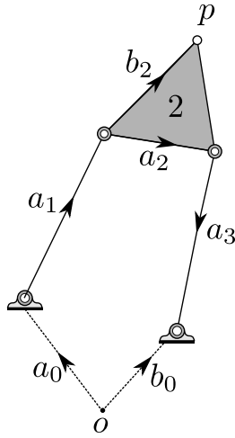
Fig. 1. Four-bar linkage
