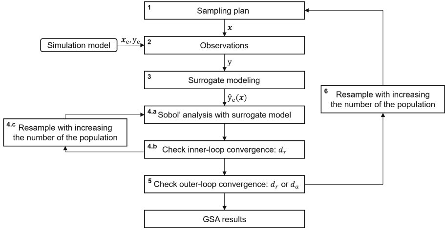
Fig. 1. flowchart of the surrogate-based iterative global sensitivity analysis algorithm.
